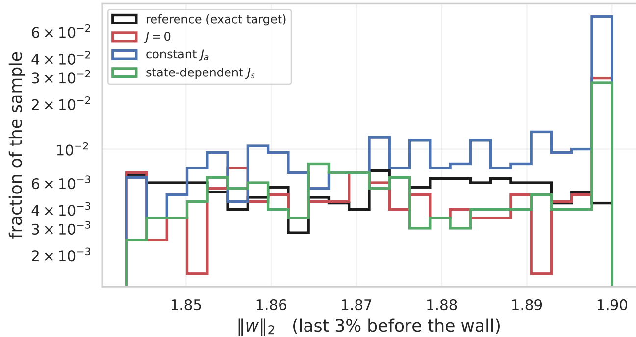
the projection atom at \|w\| = R
