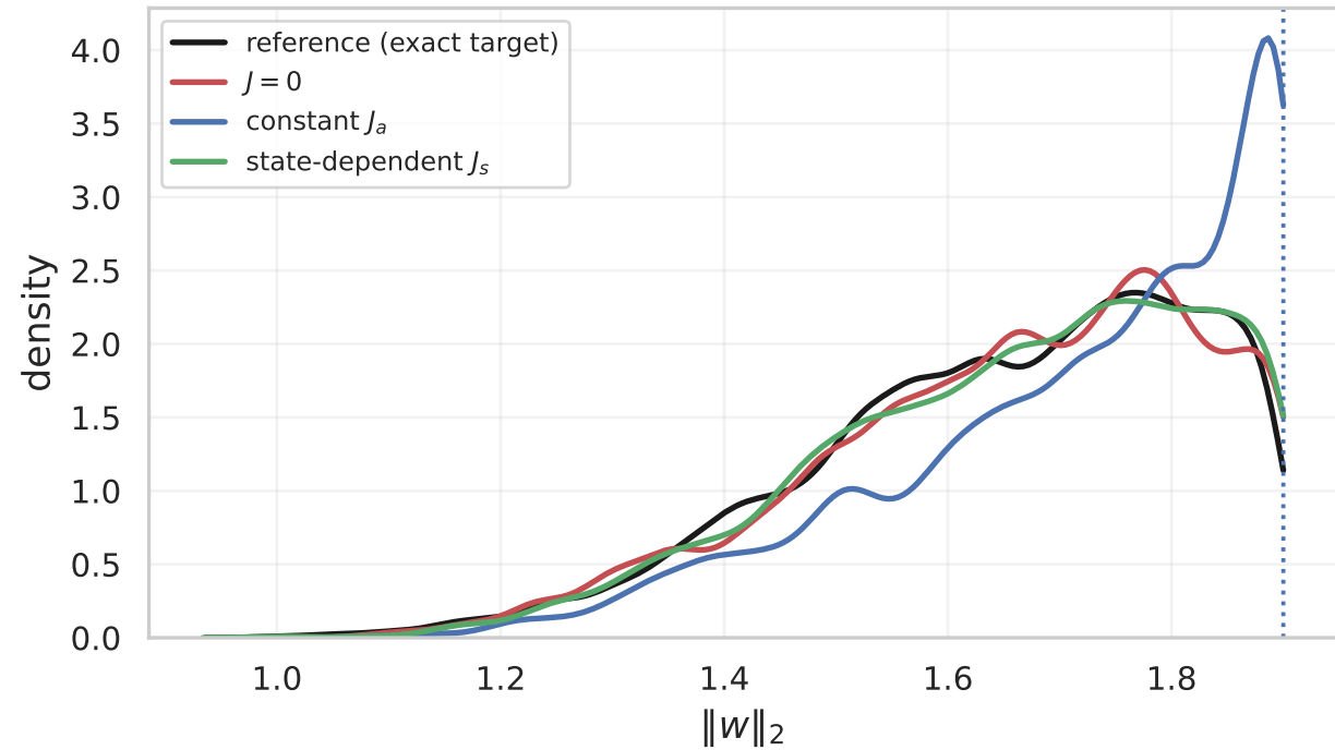
radial marginal
