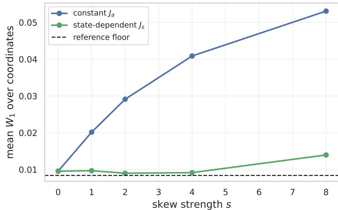
MAGIC Gamma Telescope (gamma vs hadron) — cost of violating J\nu = 0
