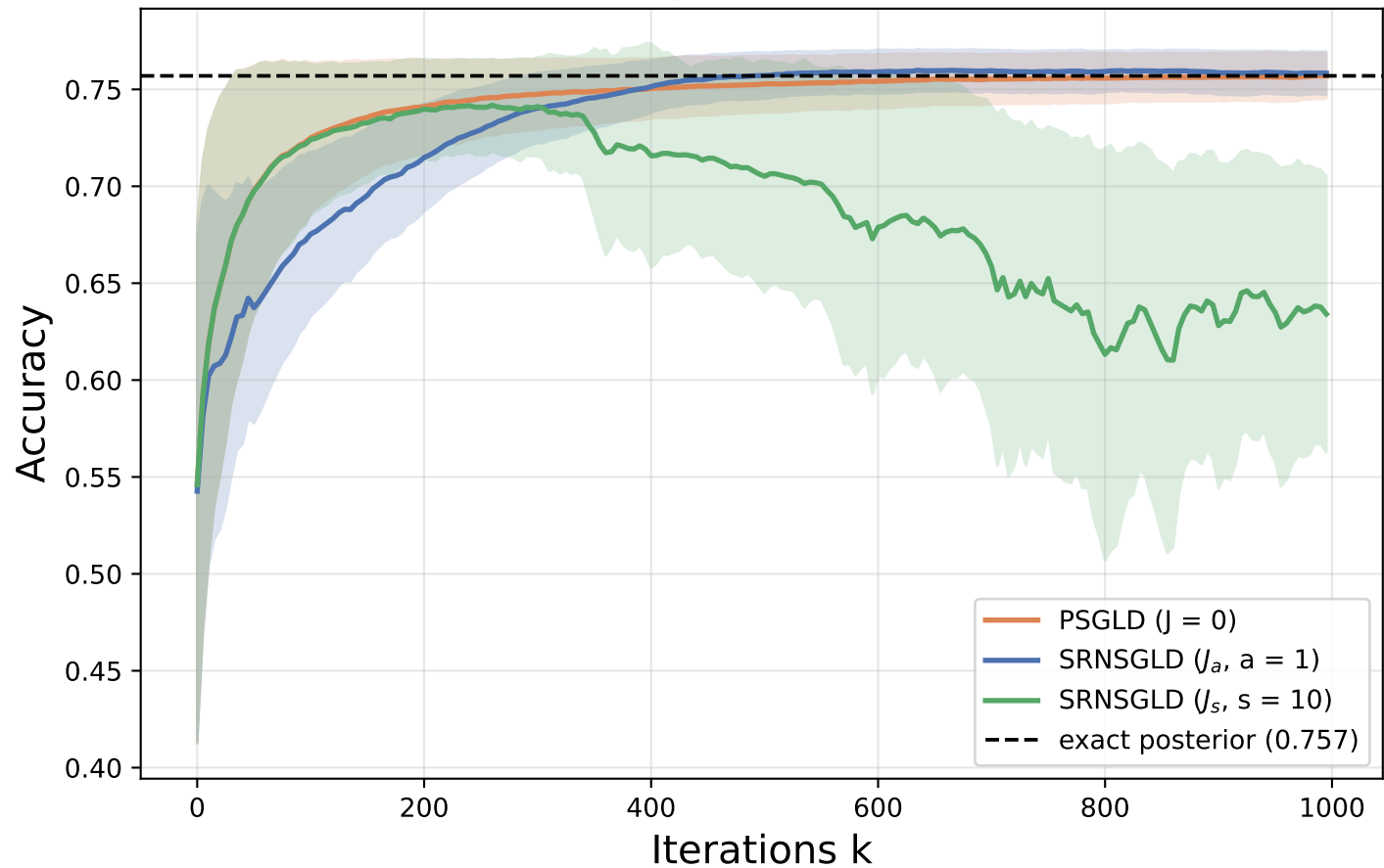
Accuracy over the test set
