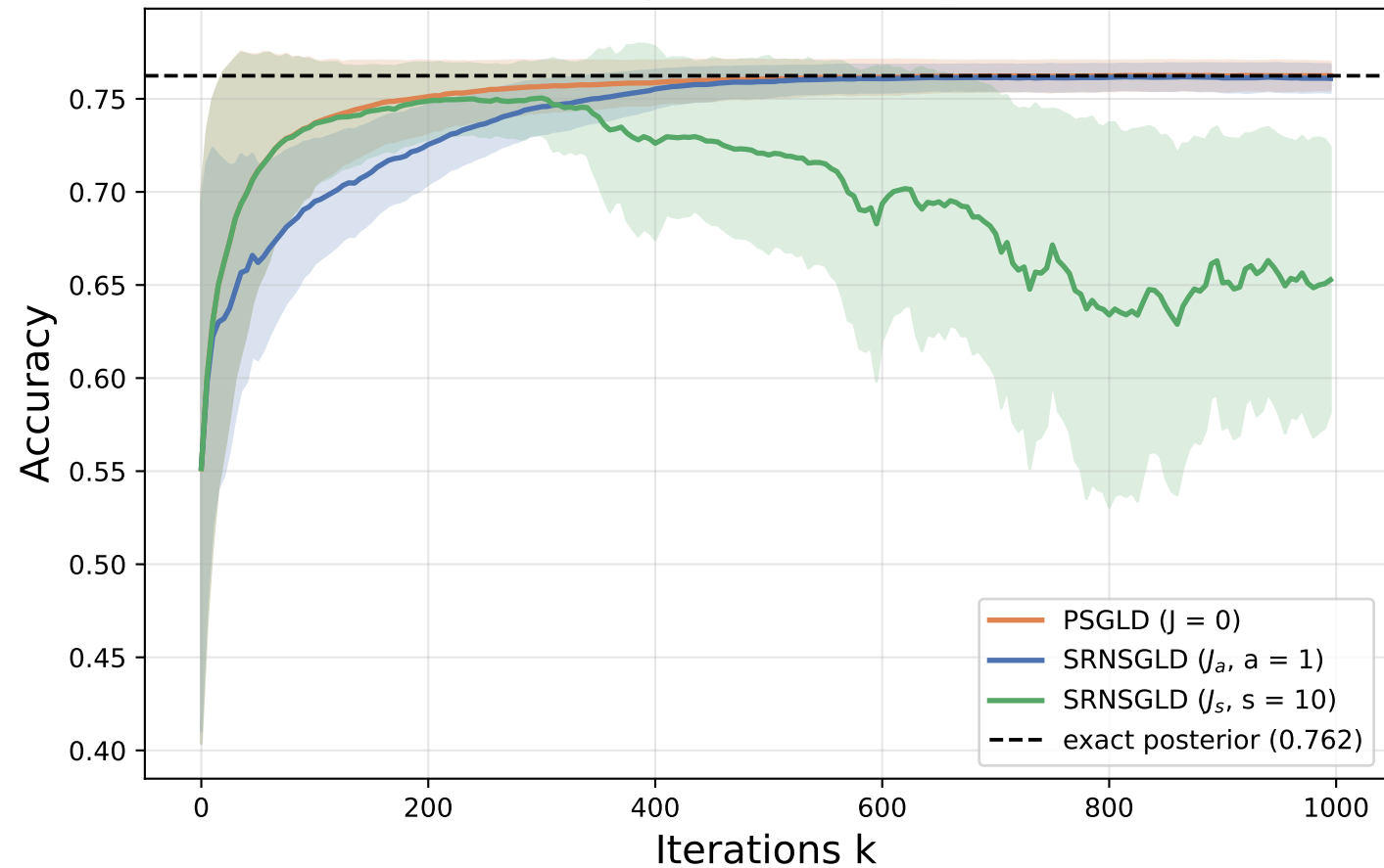
Accuracy over the training set
