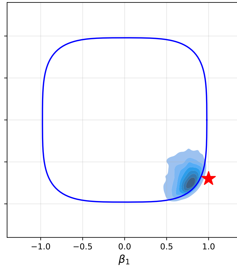
SRNSGLD (J_a, a = 1) on boundary: 7.6%
