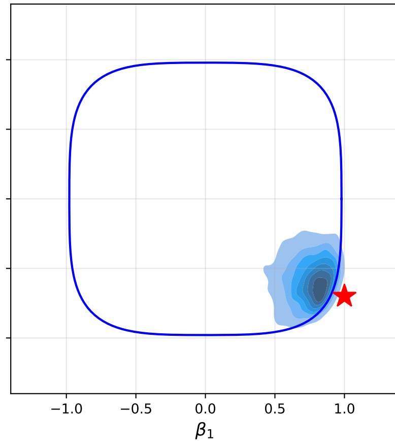
PSGLD (J = 0) on boundary: 5.3%
