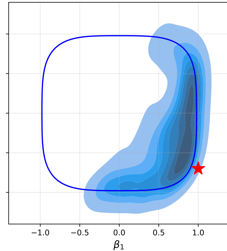
SRNSGLD (J_s, s = 10) on boundary: 32.1%
