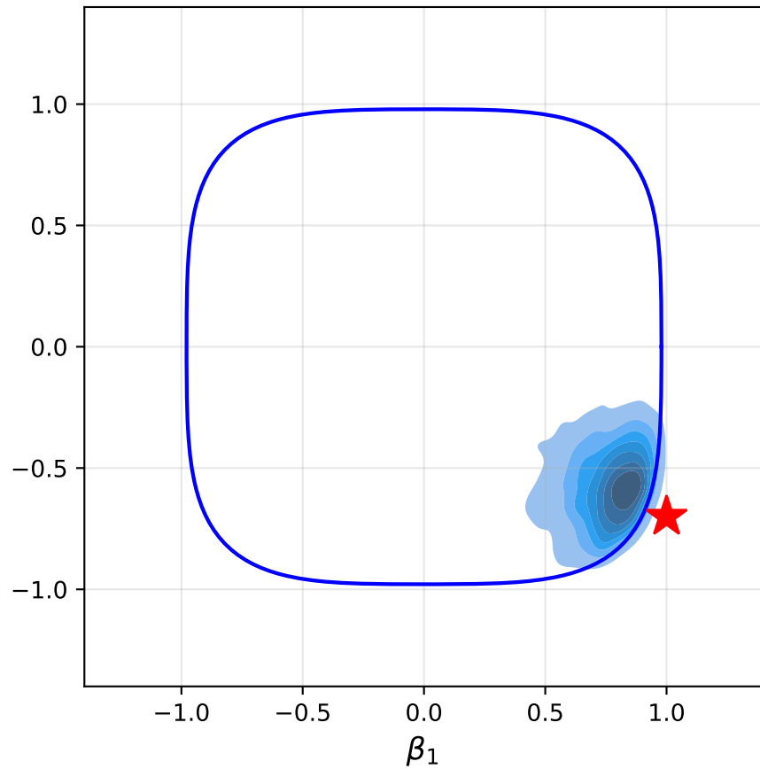
Exact posterior (grid) on boundary: 0.0%
