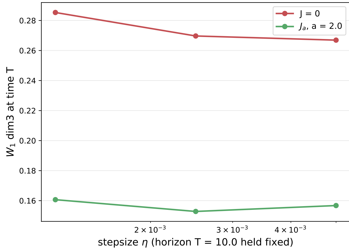
Target B: correlated \ell_1 Laplace
