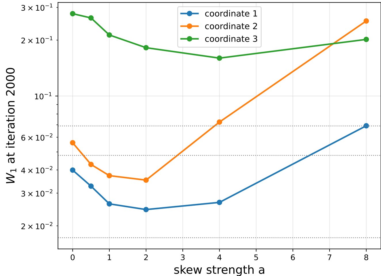
Target B: correlated \ell_1 Laplace
