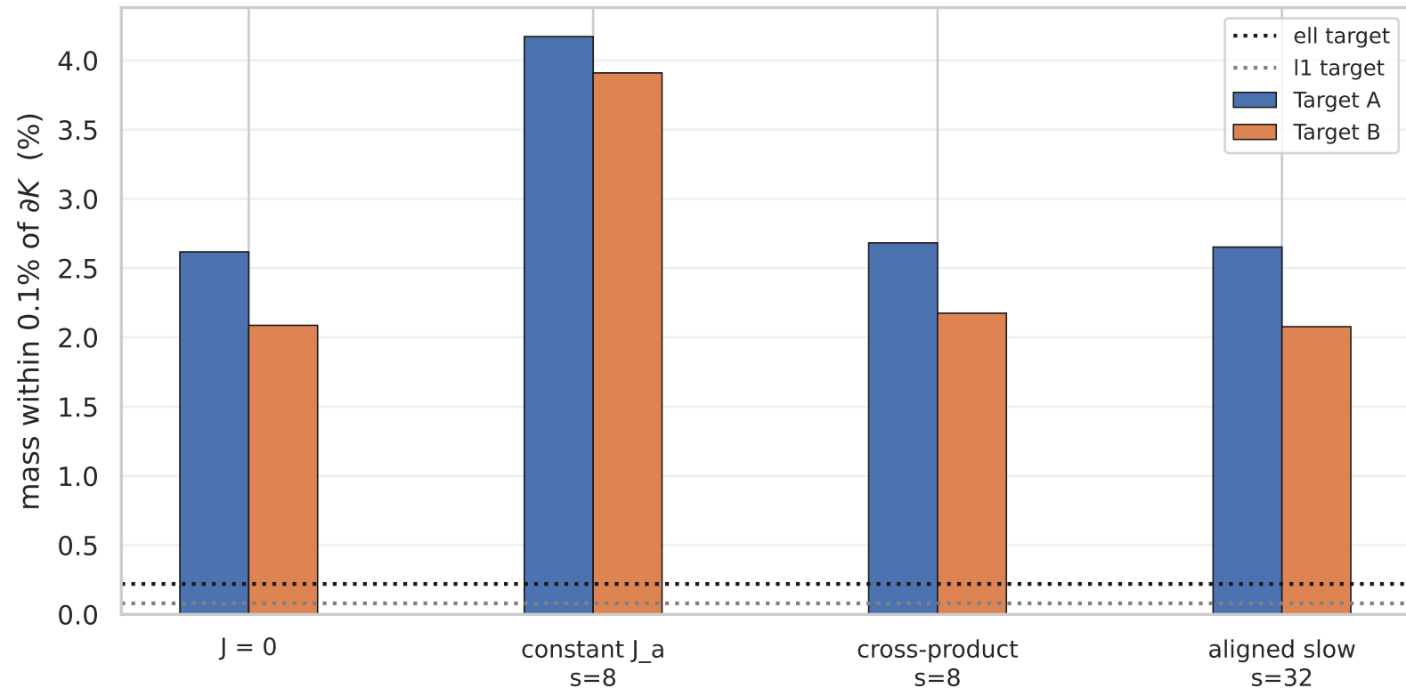
The projection atom: admissible fields leave it alone
