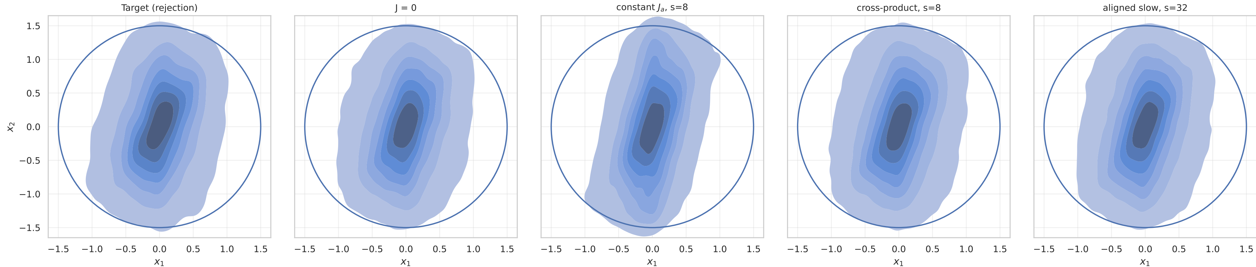
Target B: correlated \ell_1 Laplace on K — dims 1 & 2
