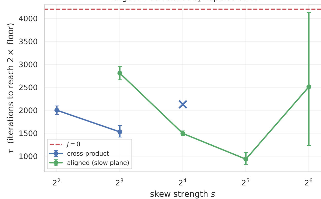
Target B: correlated \ell_1 Laplace on K
