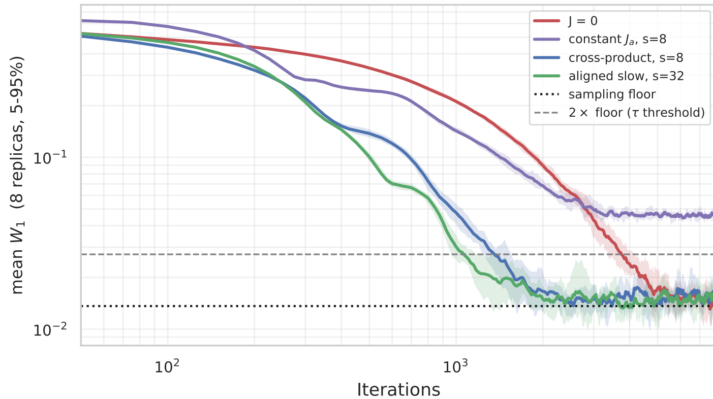
Target A: elliptical Laplace on K
