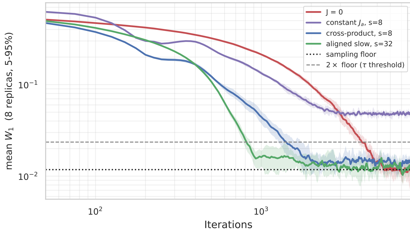
Target B: correlated \ell_1 Laplace on K
