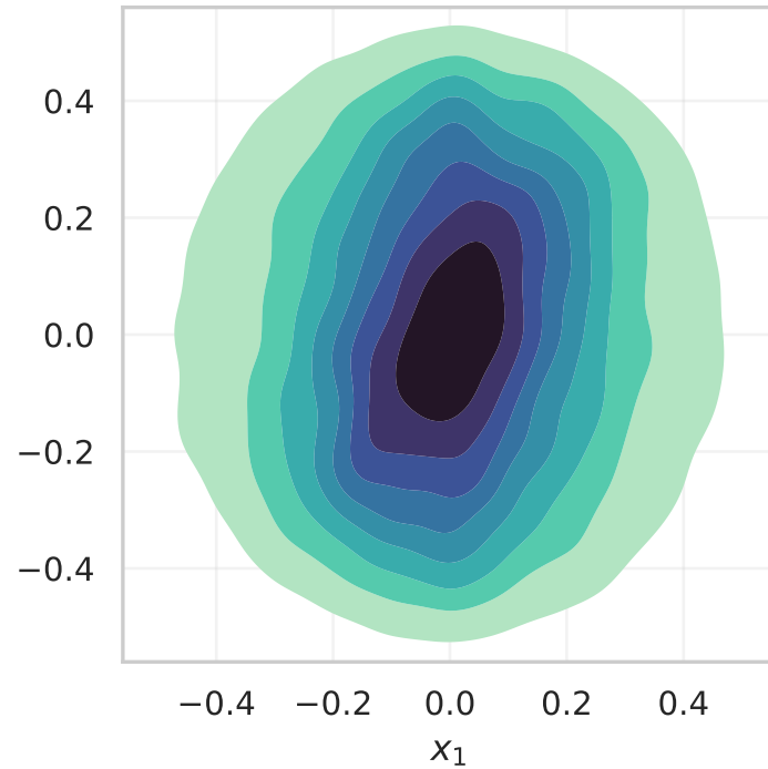
J_s, s=8
