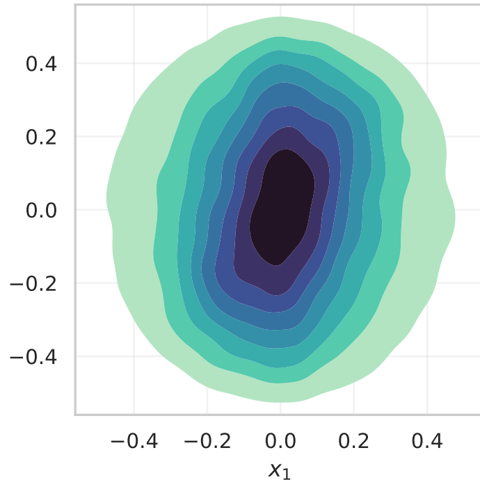
J = 0
