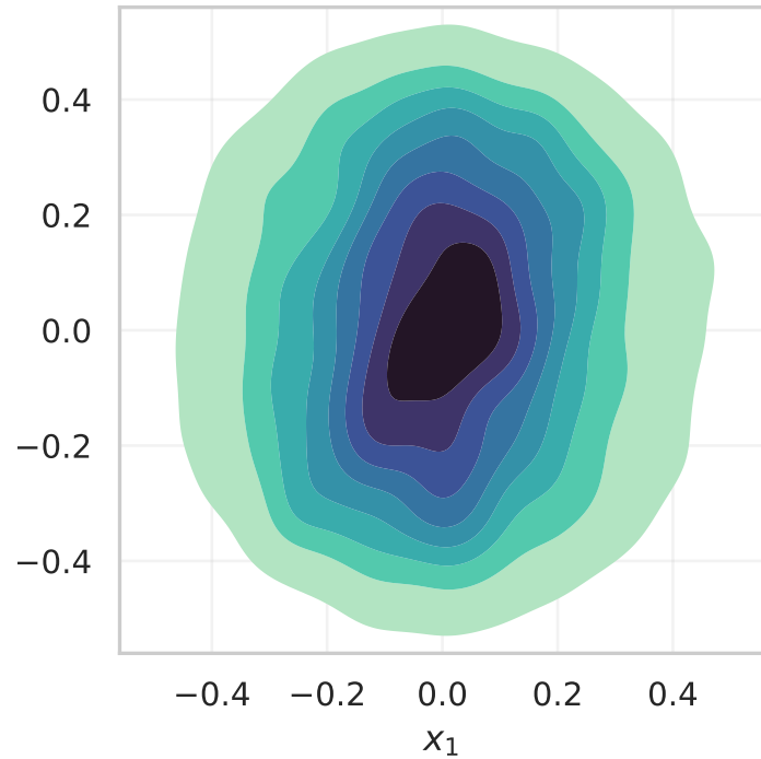
target (exact, by rejection)
