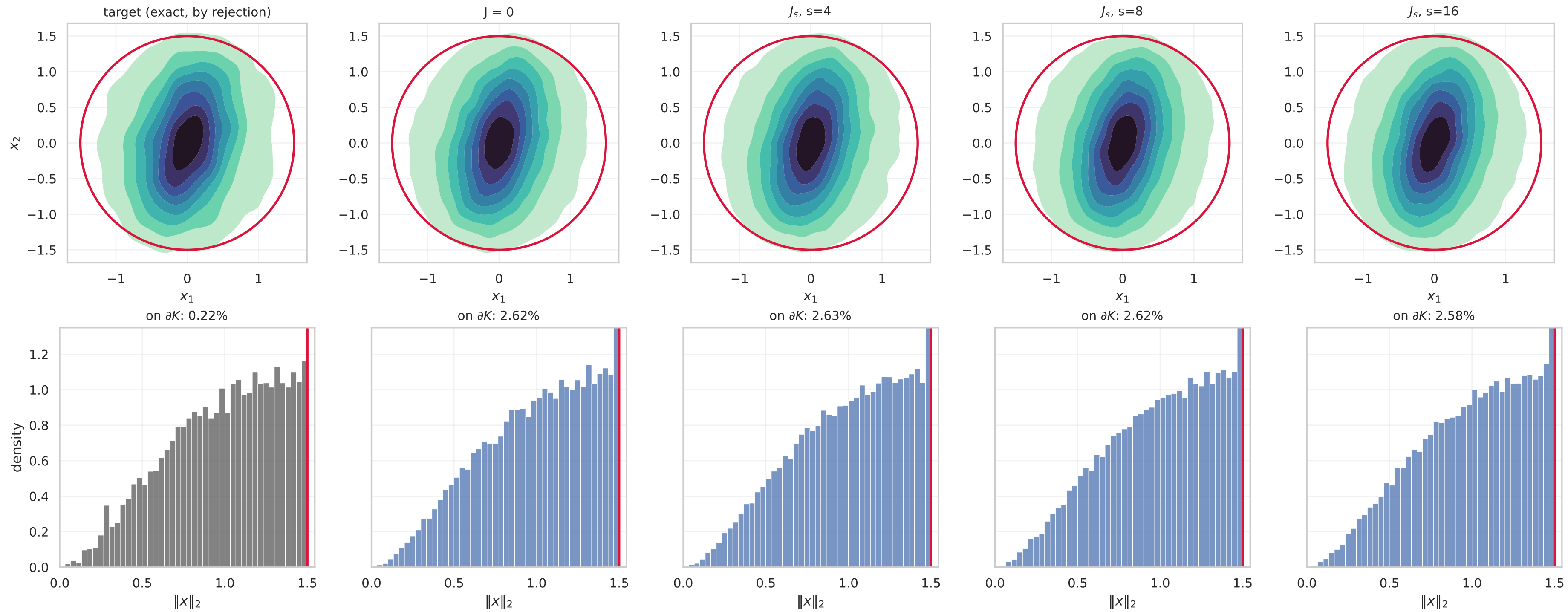
Target A: elliptical Laplace on K — the target inside K , and how each scheme fills it
