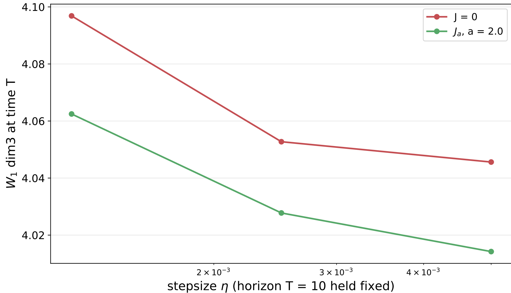
Fixed-time control
