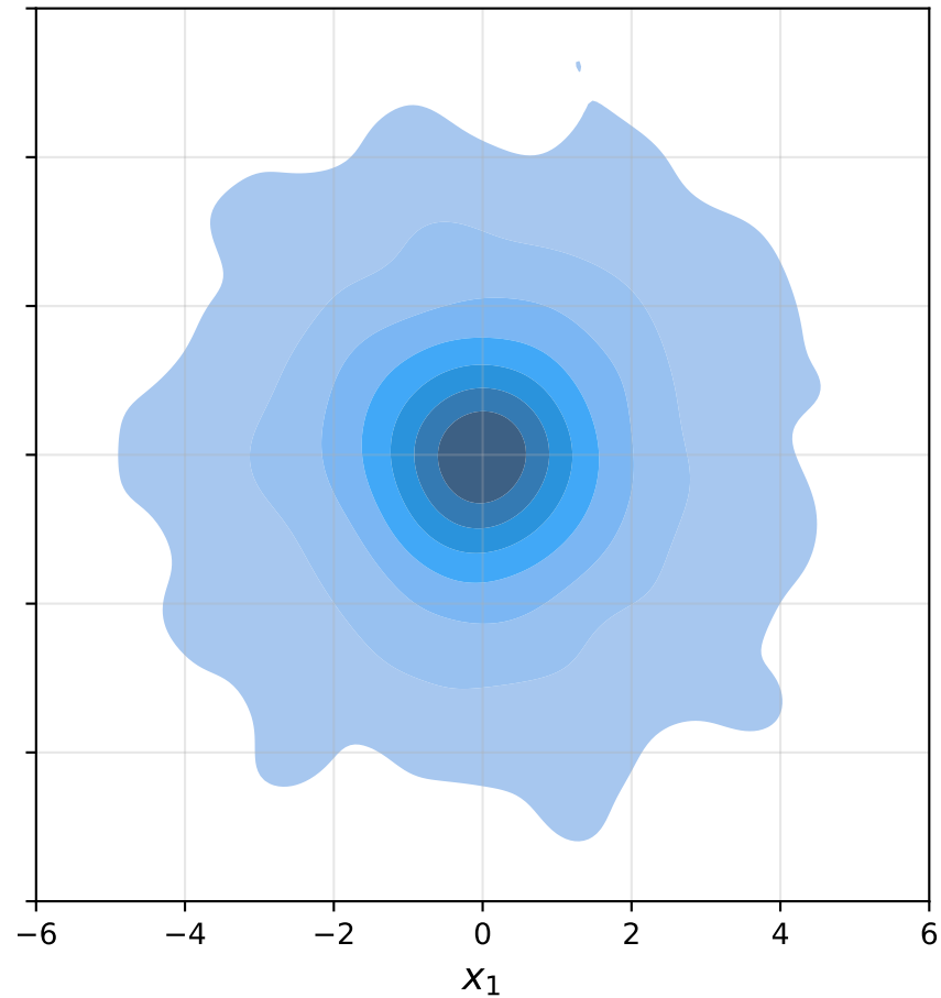
J_a, a = 2.0 (shown: |x| < 6.0 ; 85.9% of target mass)
