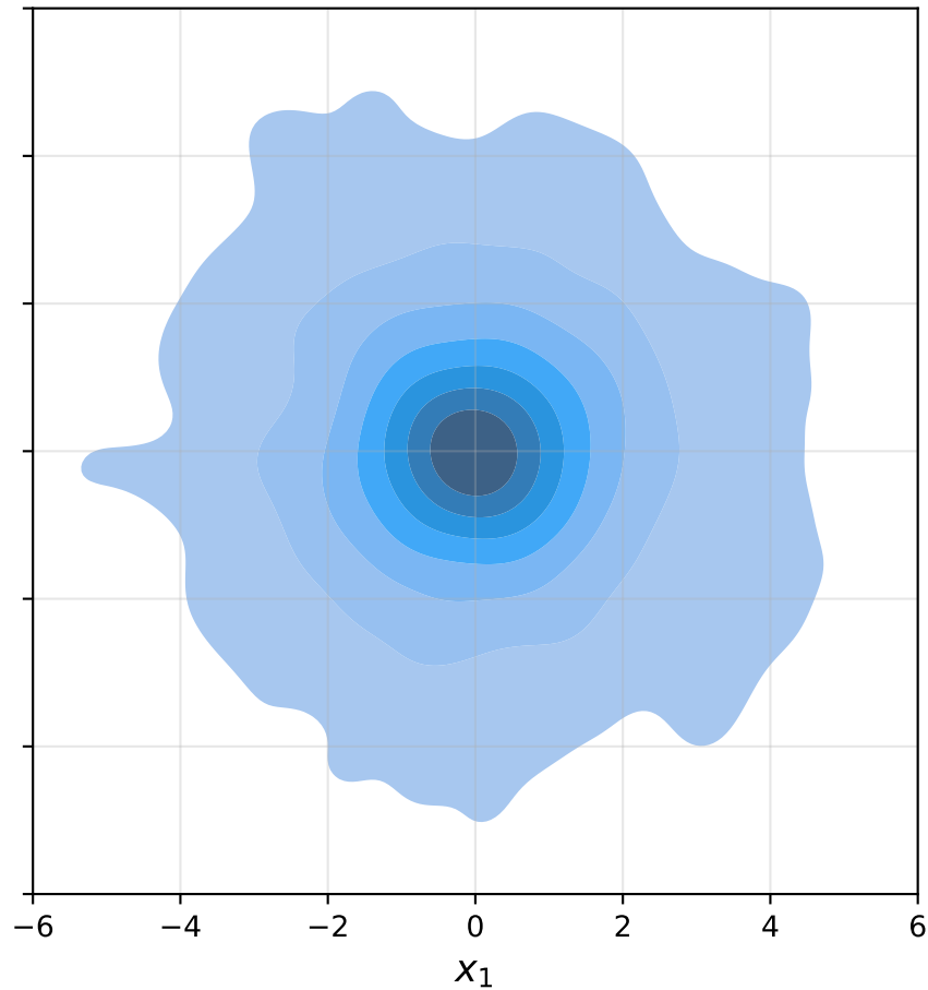
J = 0 (shown: |x| < 6.0 ; 85.9% of target mass)
