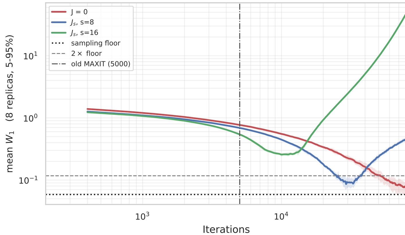
Target A: elliptical Laplace on \mathbb{R}^3
