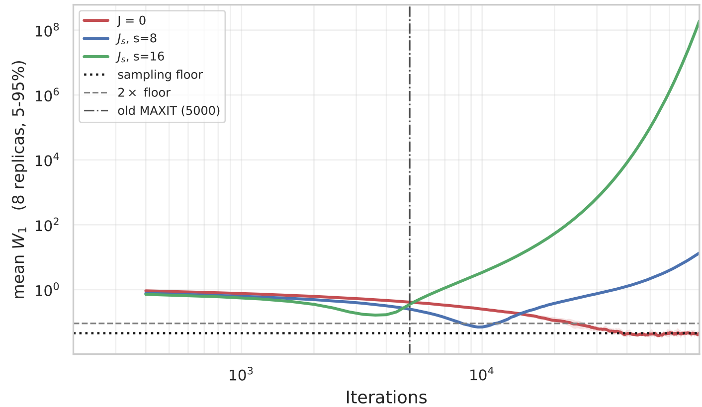
Target B: correlated \ell_1 Laplace on \mathbb{R}^3
