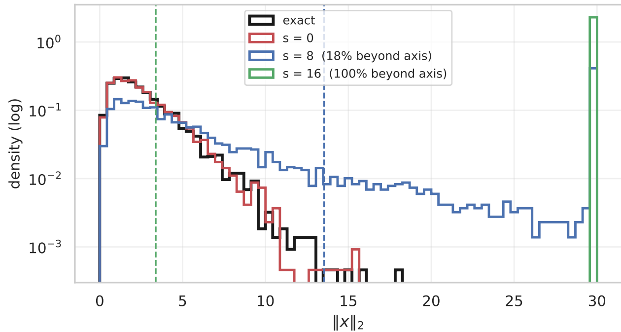
Target B: correlated \ell_1 Laplace on \mathbb{R}^3 (dashed: r^* )
