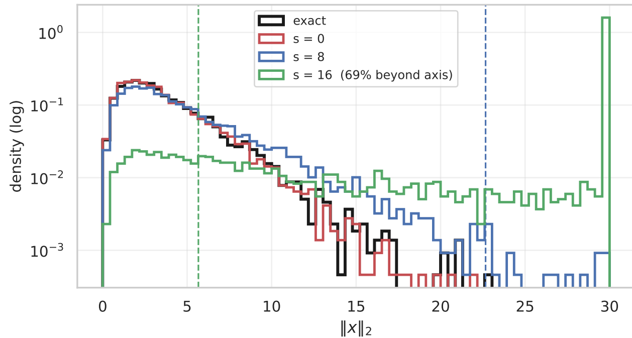
Target A: elliptical Laplace on \mathbb{R}^3 (dashed: r^* )
