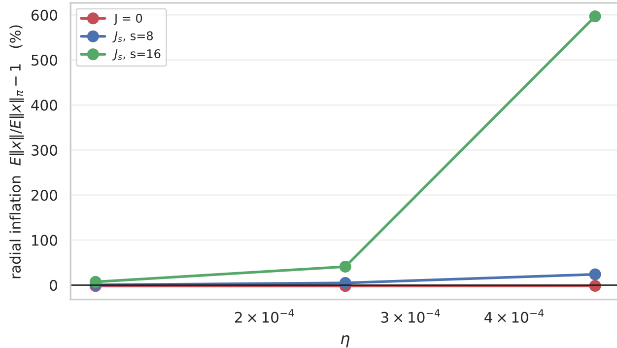
Target A: elliptical Laplace on \mathbb{R}^3
