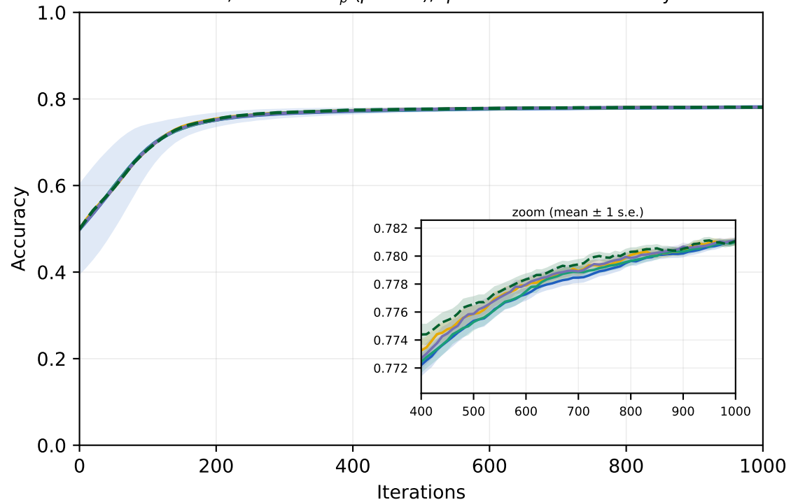
MAGIC, smoothed \ell_p ( p = 2.4 ), \eta = 1e-06 -- test accuracy
