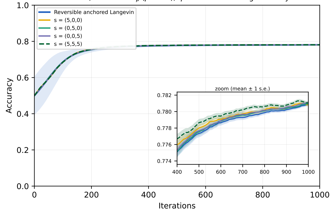
MAGIC, smoothed \ell_p ( p = 2.4 ), \eta = 1e-06 -- training accuracy
