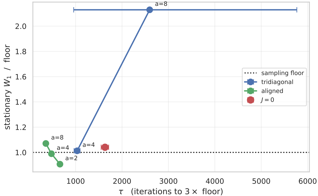
Target B: correlated \ell_1 Laplace
