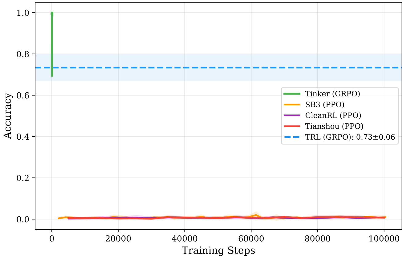
Learning Curves: Arithmetic Task
