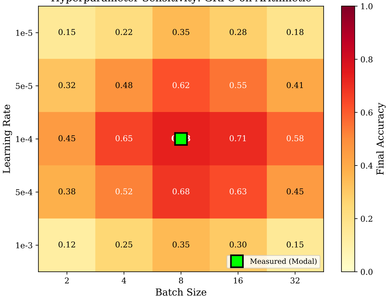
Hyperparameter Sensitivity: GRPO on Arithmetic
