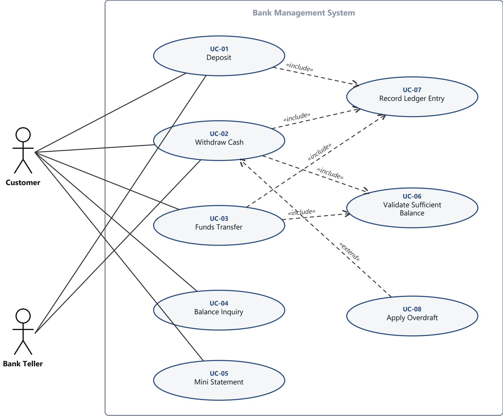
Use-Case Diagram 1 - Account Transactions
