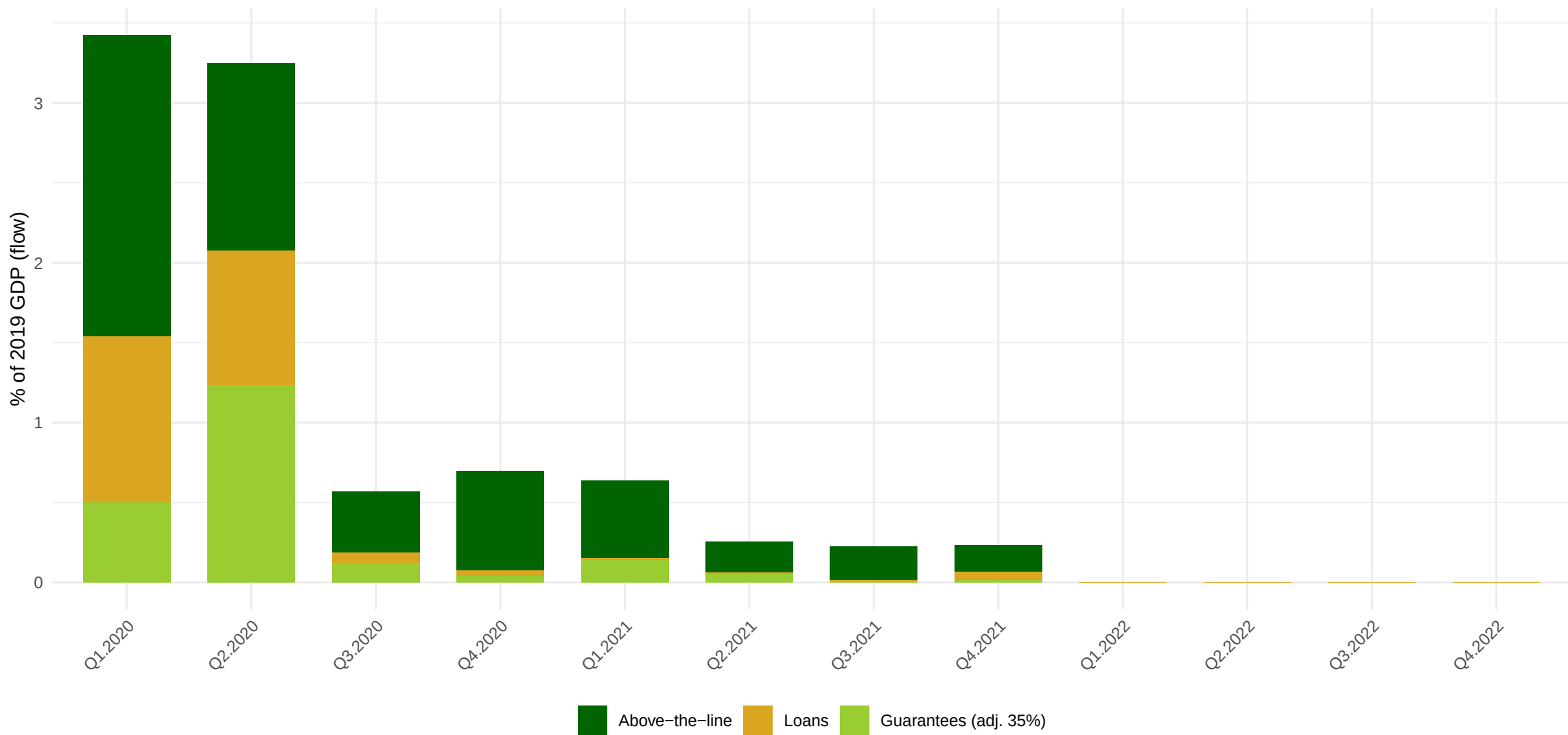
CP Decomposition per Quarter
