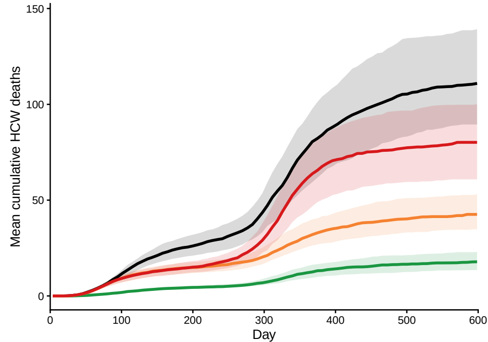
Delayed coverage + dosing analysis (optimistic efficacy)
