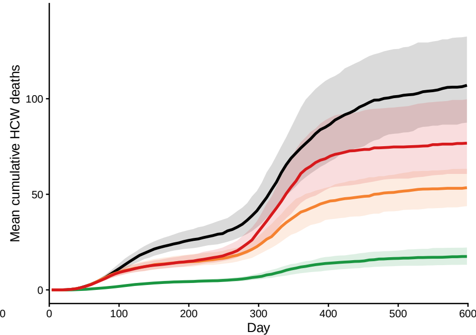
Delayed coverage + dosing analysis (central efficacy)
