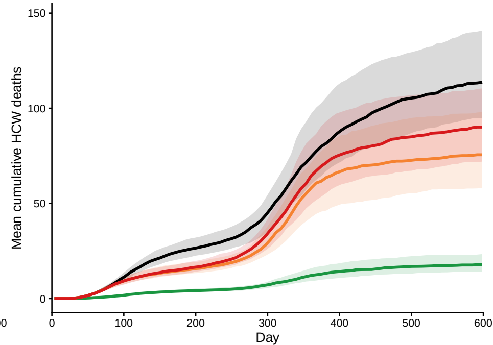
Delayed coverage + dosing analysis (pessimistic efficacy)
