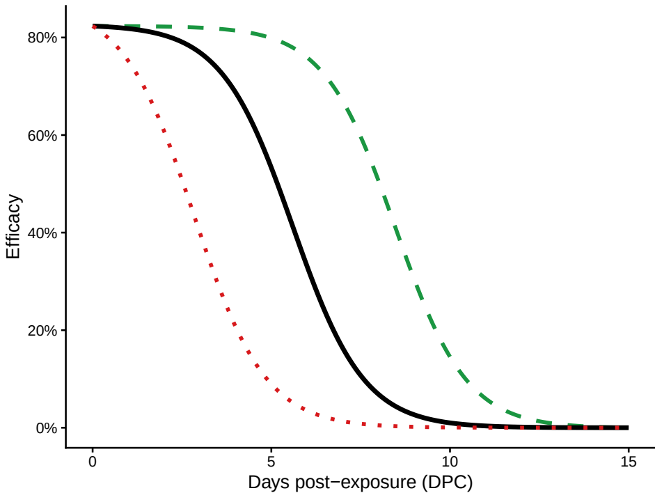
Efficacy vs days post-exposure (DPC)
