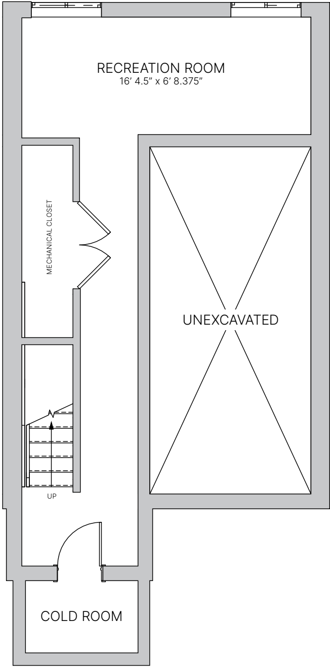
BASEMENT
