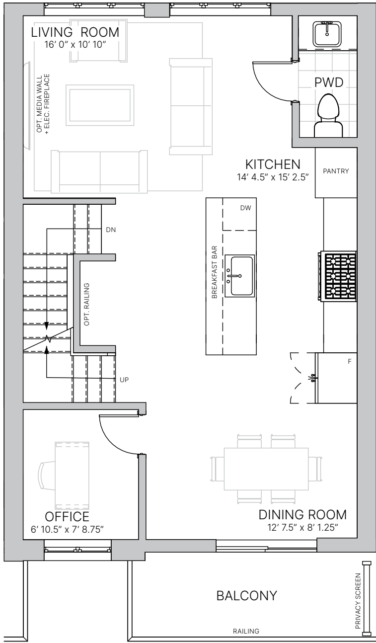
SECOND FLOOR
