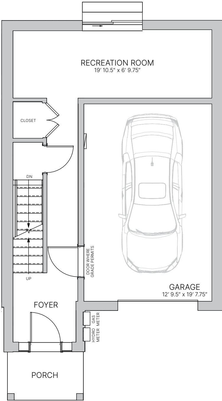
FIRST FLOOR
