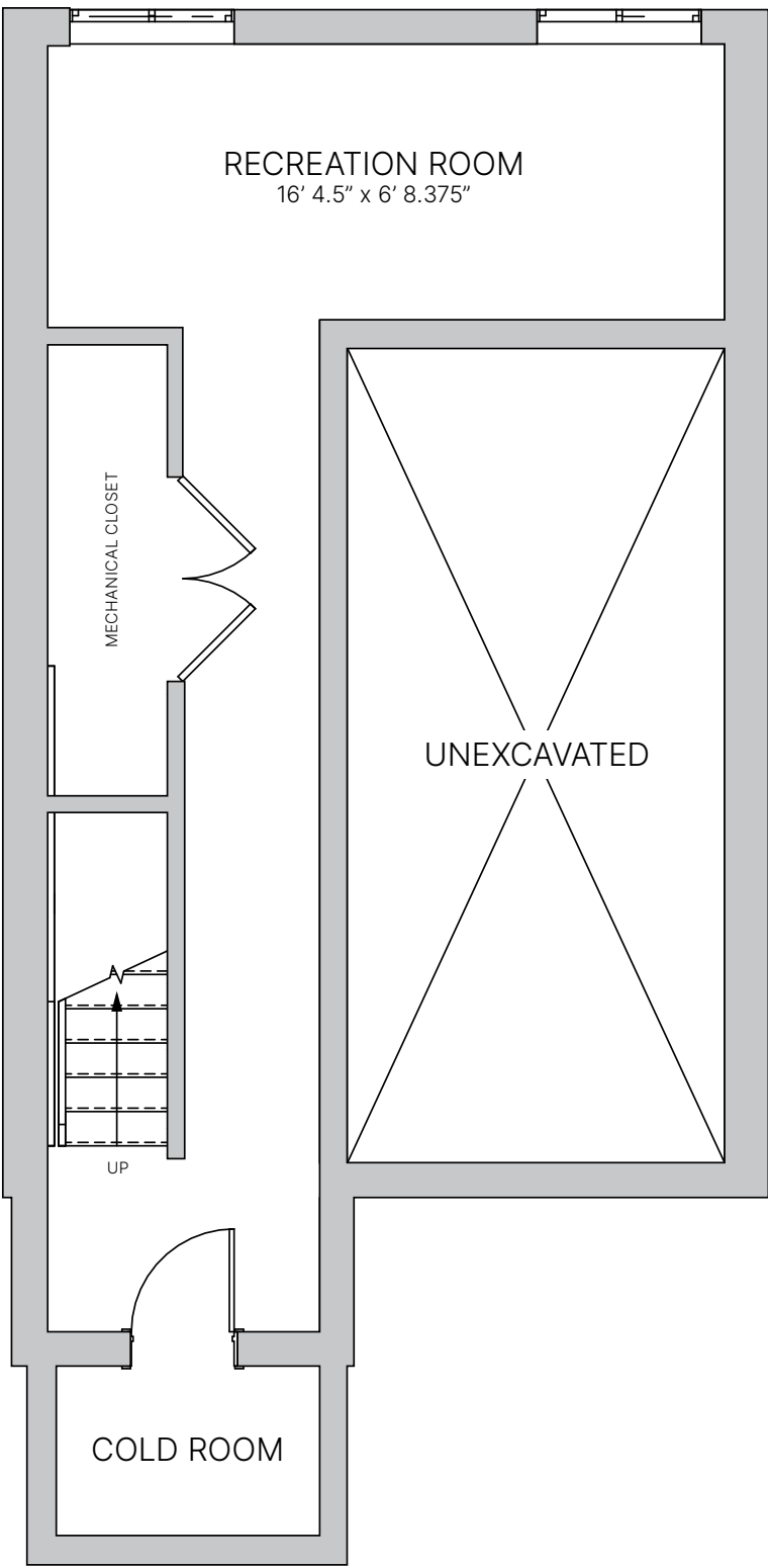
BASEMENT
