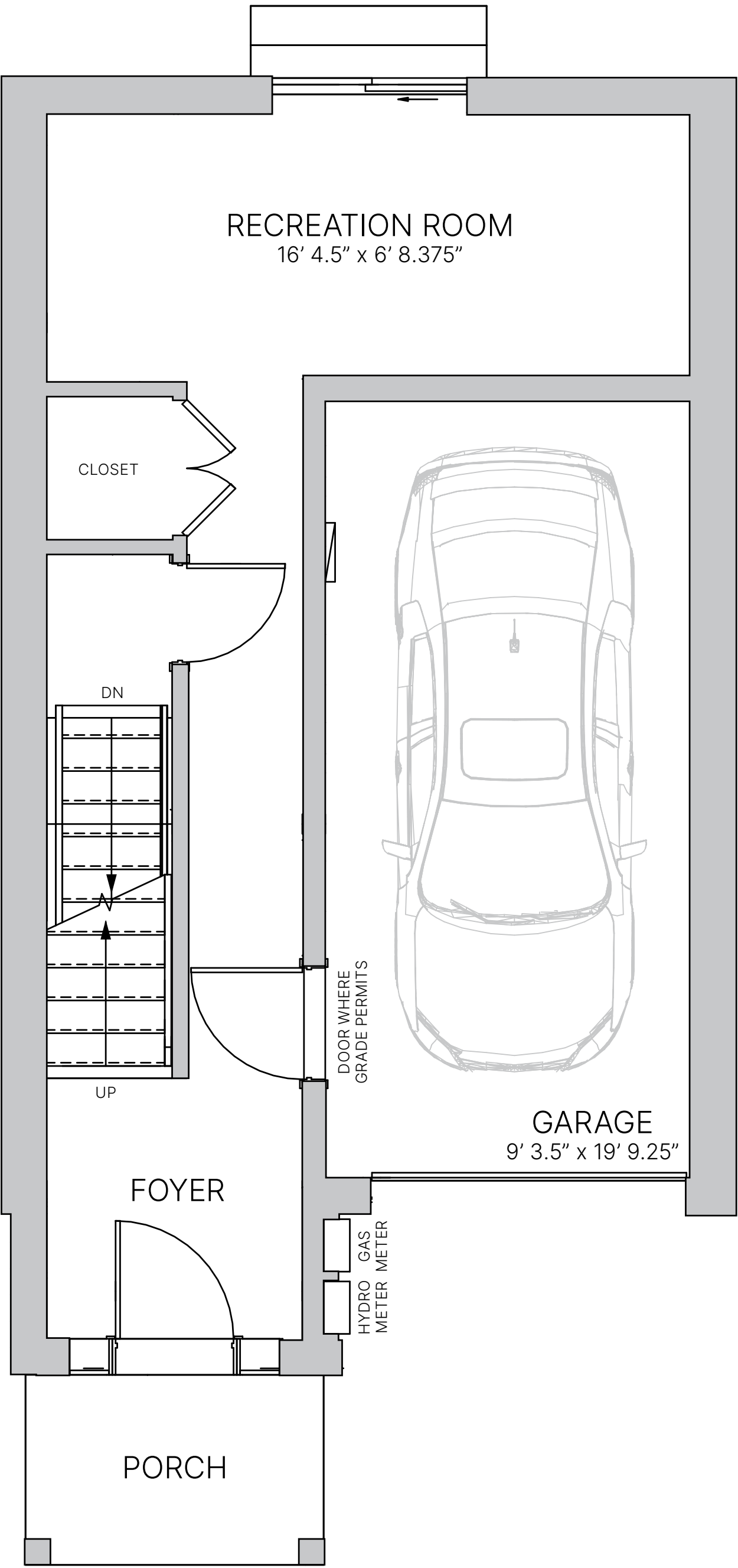
FIRST FLOOR
