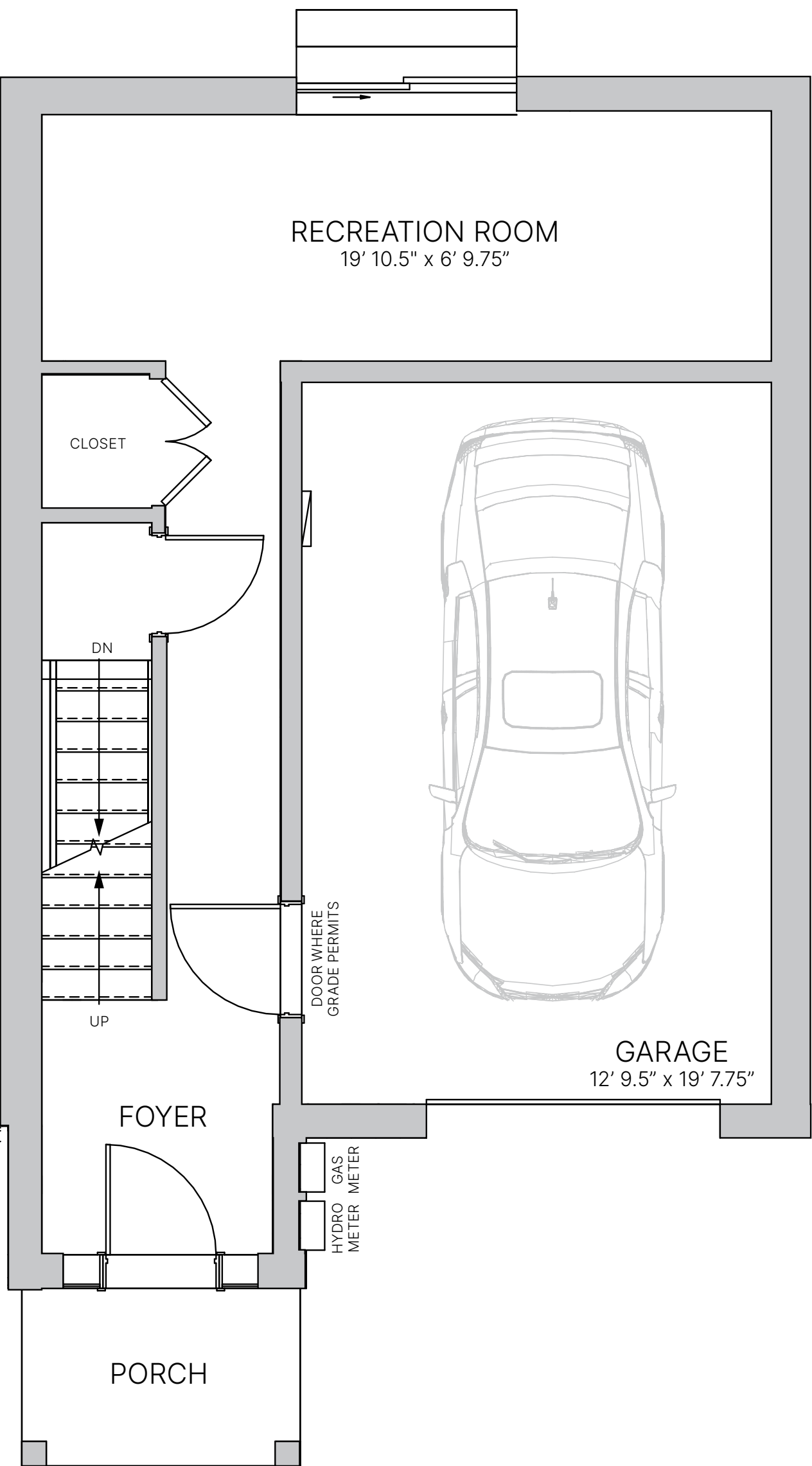
FIRST FLOOR
