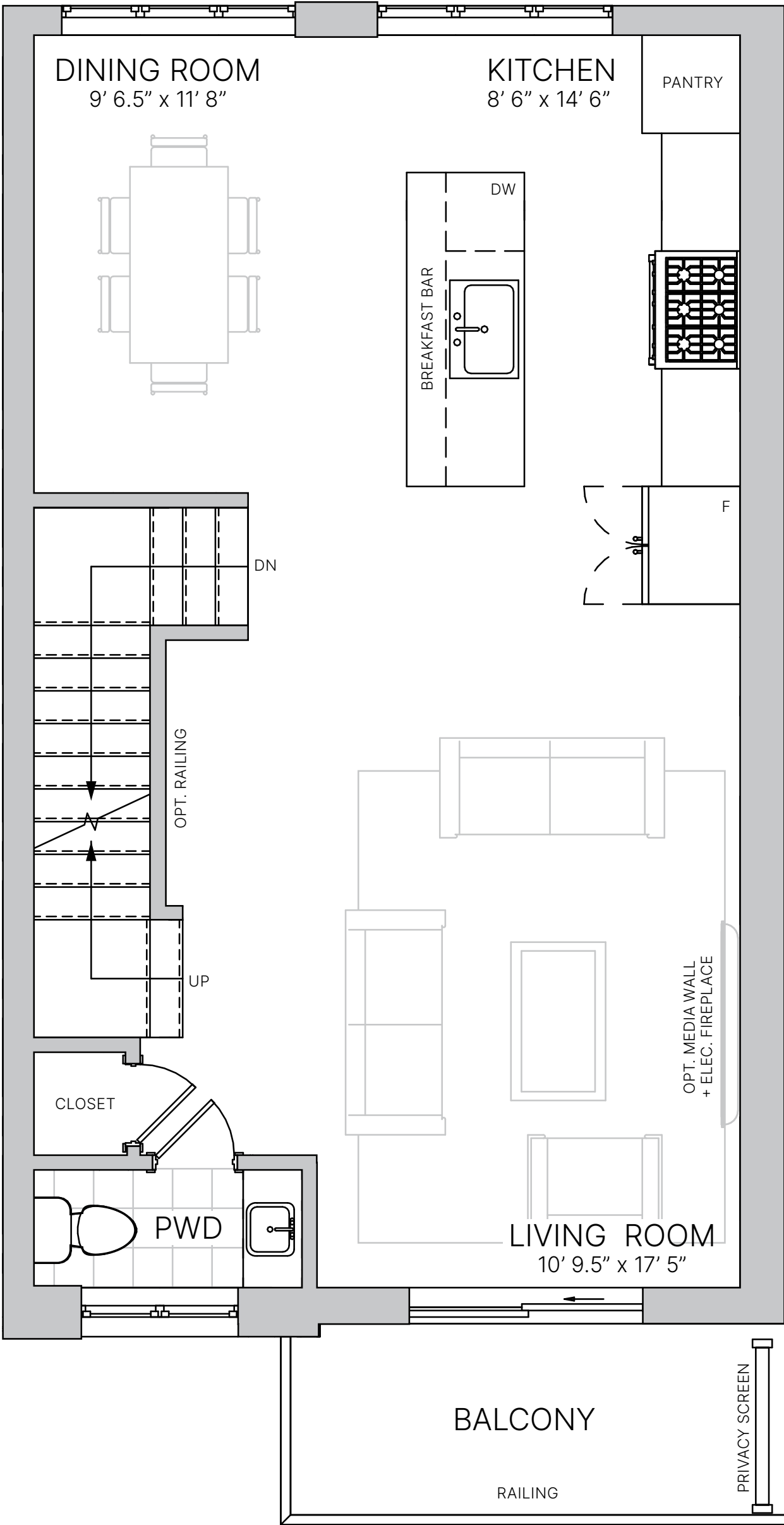
SECOND FLOOR
