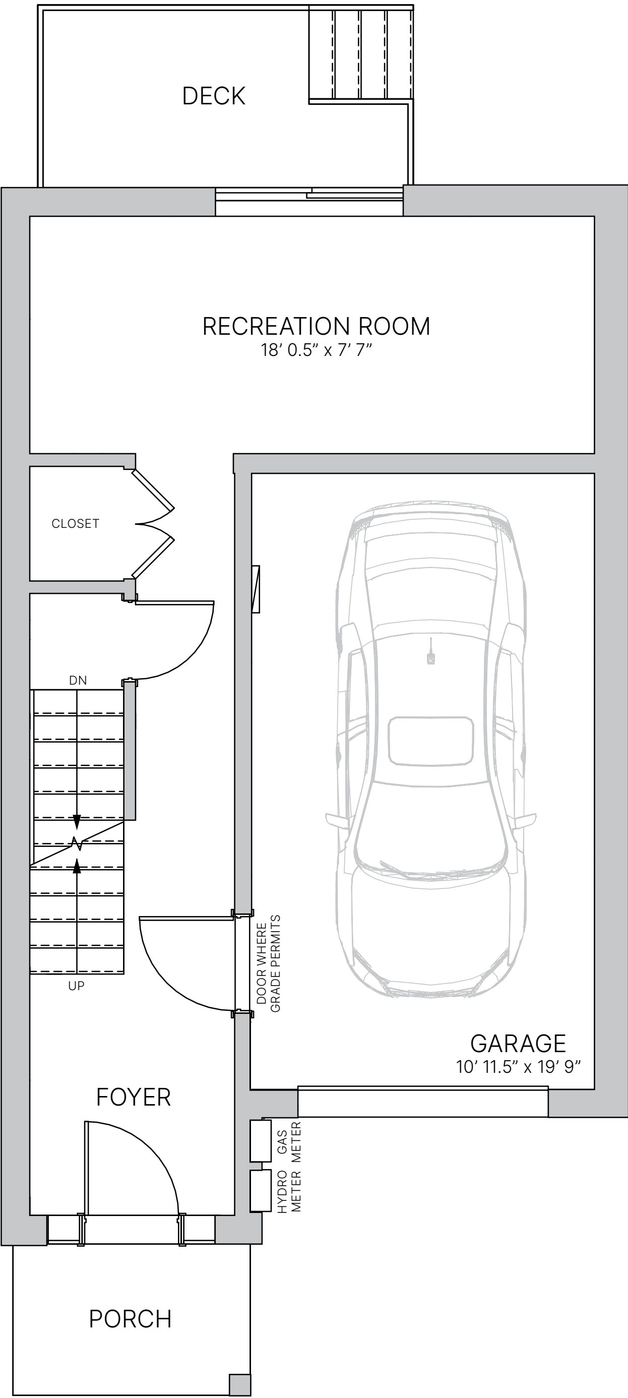
FIRST FLOOR
