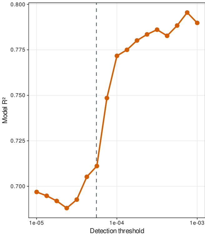
B. Abundance-occupancy fit
