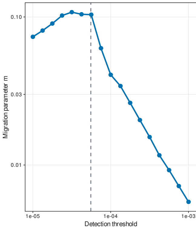
A. Migration estimate
