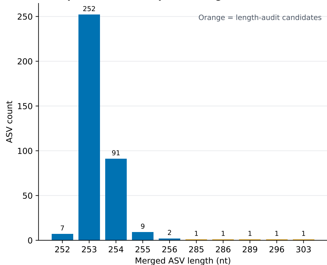
A Representative-sequence lengths
