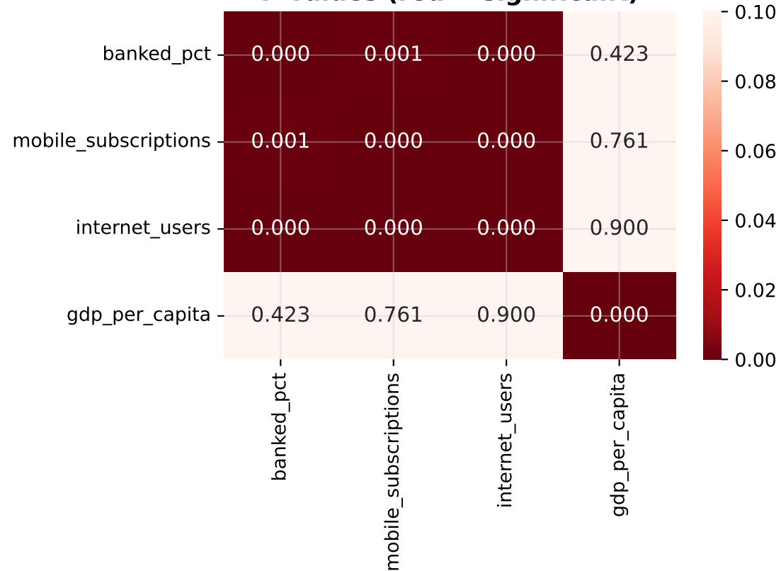
P-values (red = significant)
