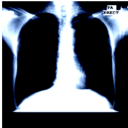
Train aug #2
