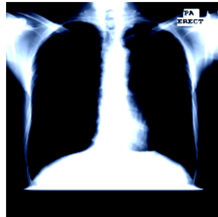
Train aug #3
