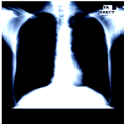
Train aug #1
