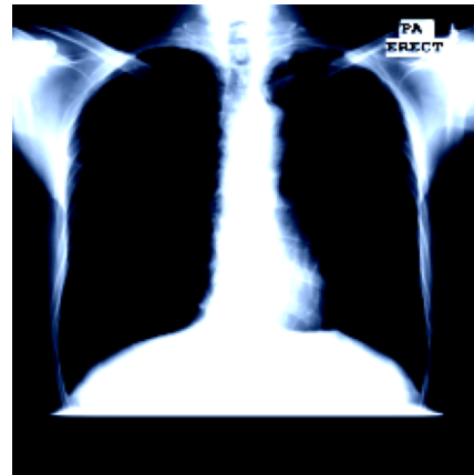
Train aug #4
