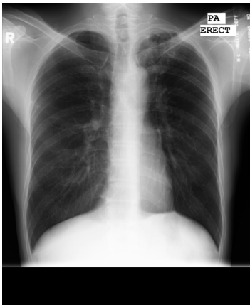
Original (grayscale)
