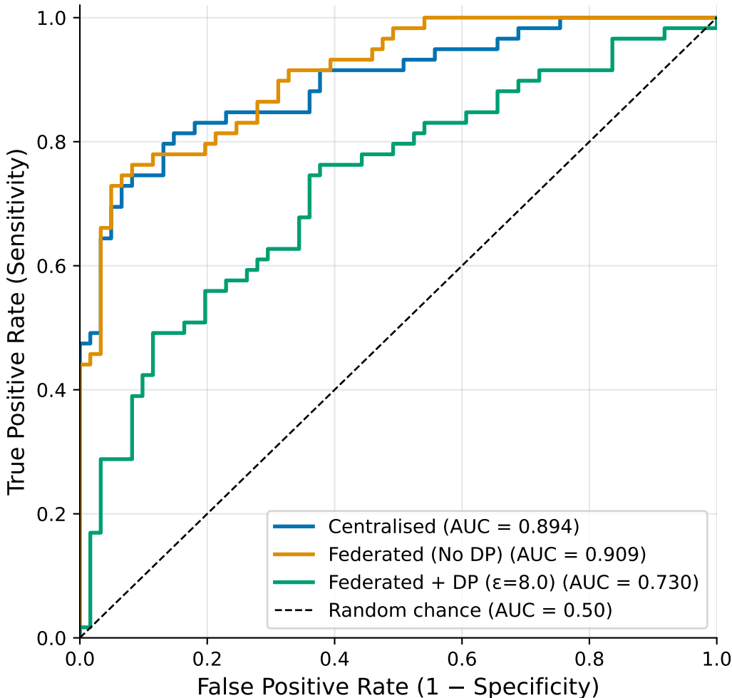
ROC Curves: Centralised vs Federated vs Federated+DP (95% CIs shown in Table 1)
