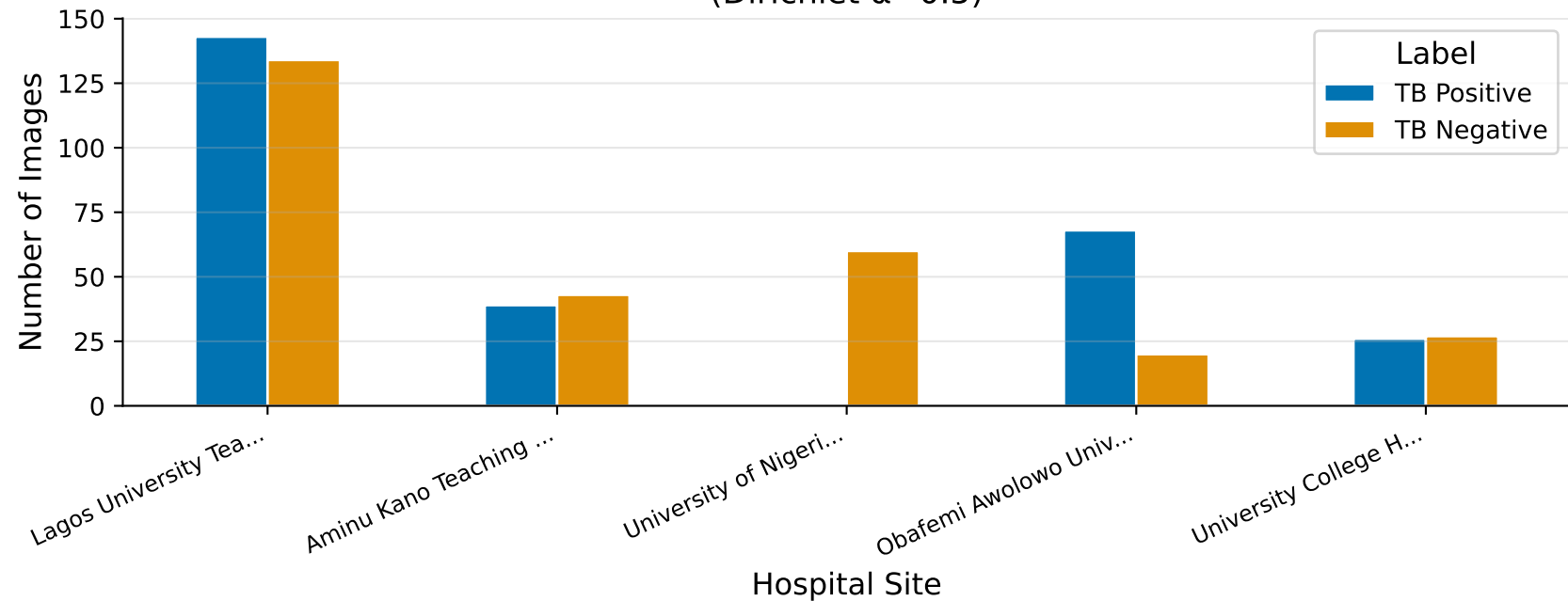
Class Distribution Across Simulated Hospital Sites (Dirichlet \alpha=0.5 )
