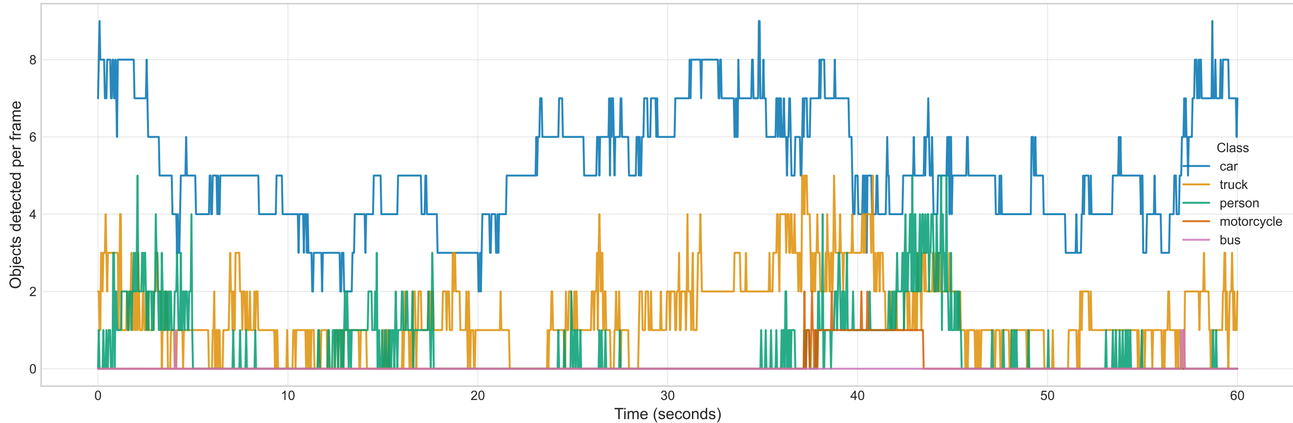
Object Count Over Time — Top 5 Classes (YOLOv8-small)
