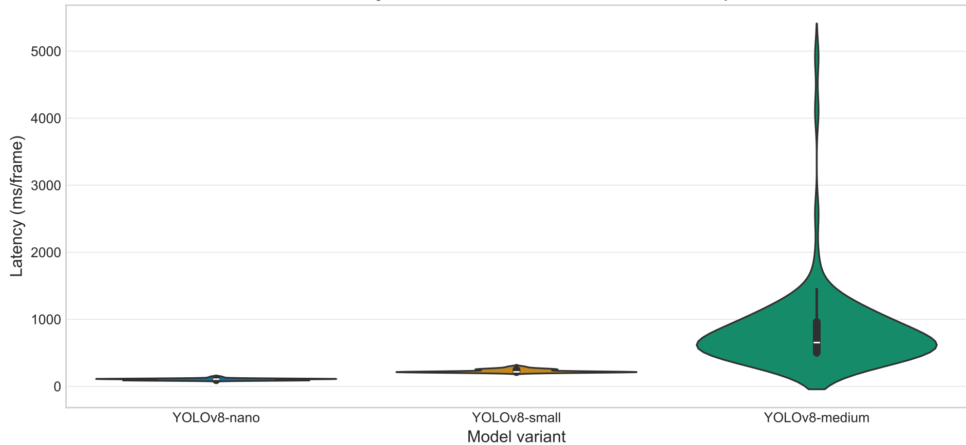
Per-Frame Latency Distribution — 100 Benchmark Frames per Model
