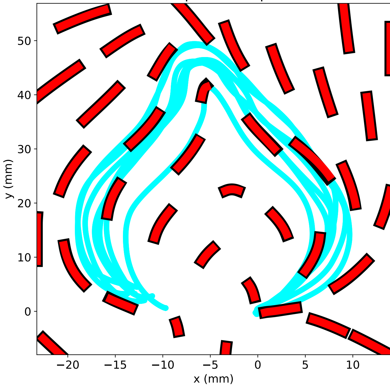
Diffeomorphism Comparison
