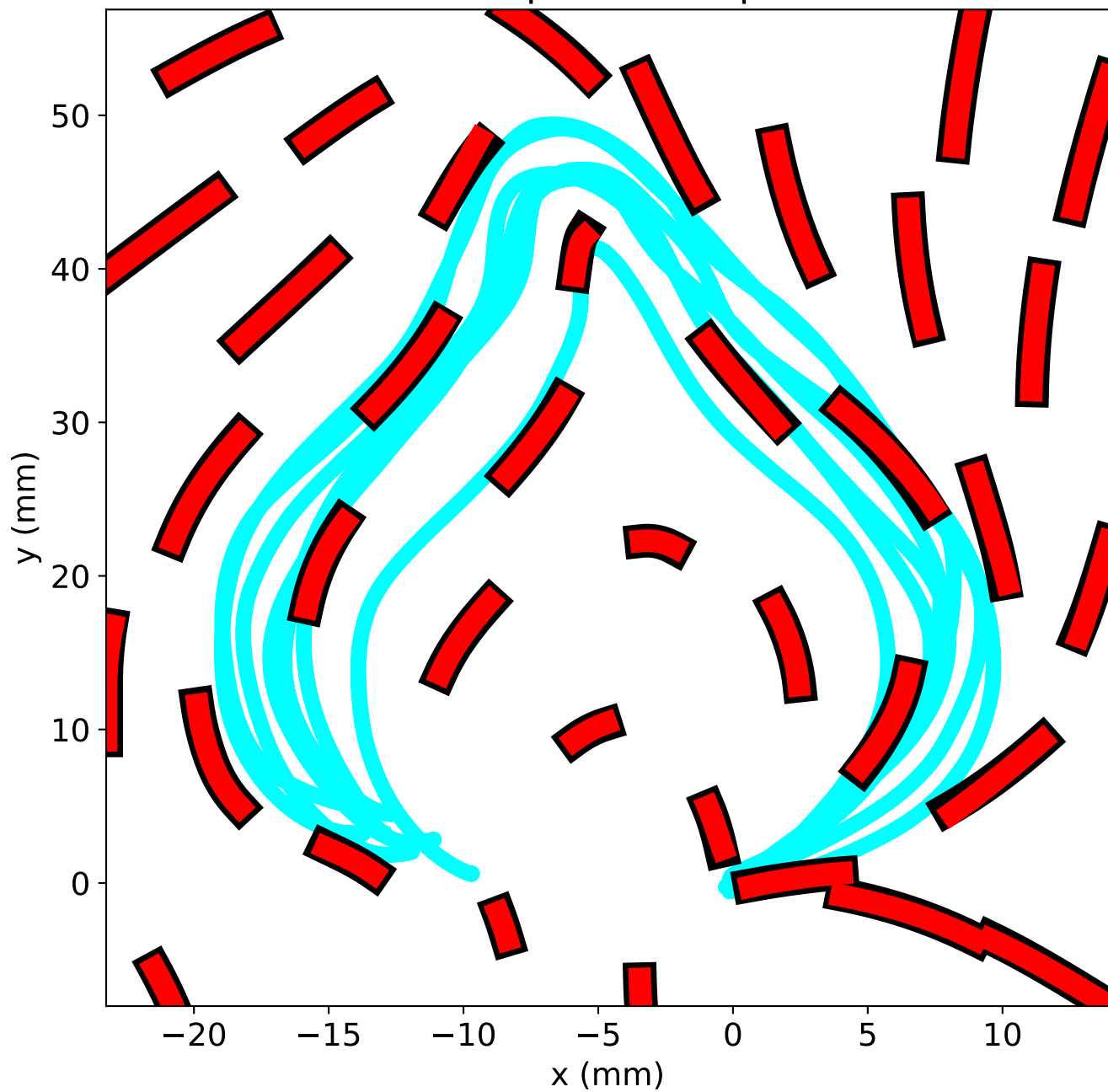
Diffeomorphism Comparison
