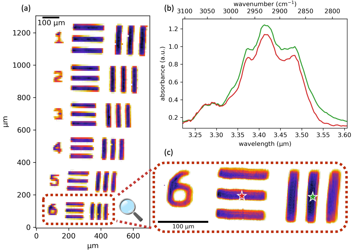
FIG. 4. Dual-comb hyperspectral image of SU-8 USAF test pattern on Silicon. (a) False-color image generated from the integrated absorbance around 2930\text{ cm}^{-1} taken at 5\text{ }\mu\text{m} spatial sampling. (b) Absorbance curves taken at the red and green points (stars) of frame (c), which is a zoomed image taken at 1.2\text{ }\mu\text{m} spatial sampling.
