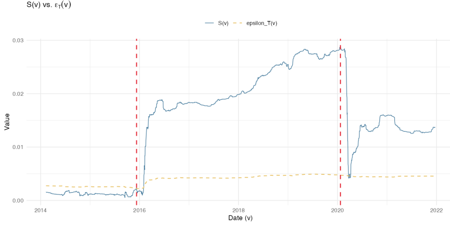
Figure 2: Localization profile S(v) (solid) against the threshold \varepsilon_T(v) (dashed) for first differenced HY OAS.
