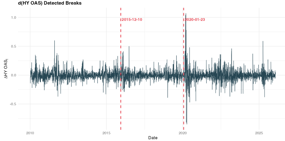
Figure 1: First differenced HY OAS over the full sample, with the two PPD-detected breaks marked
