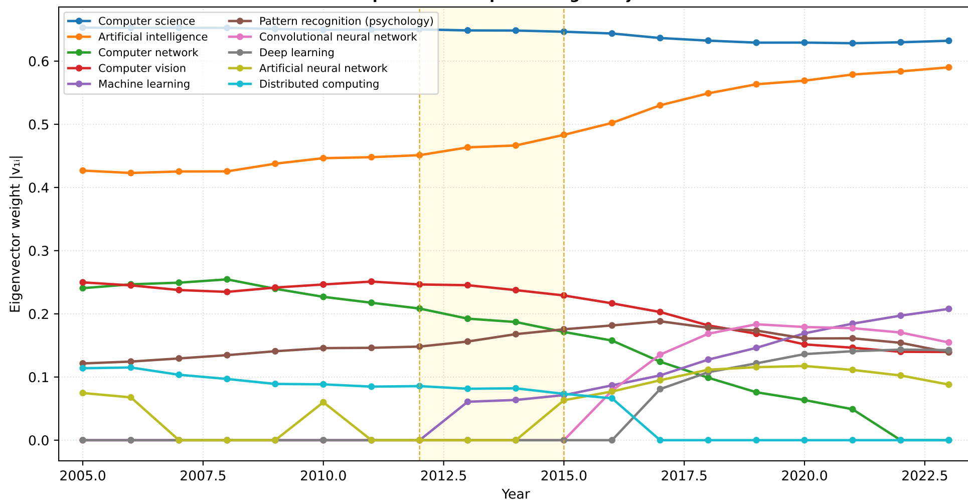
B Top-10 CS concepts — weight trajectories
