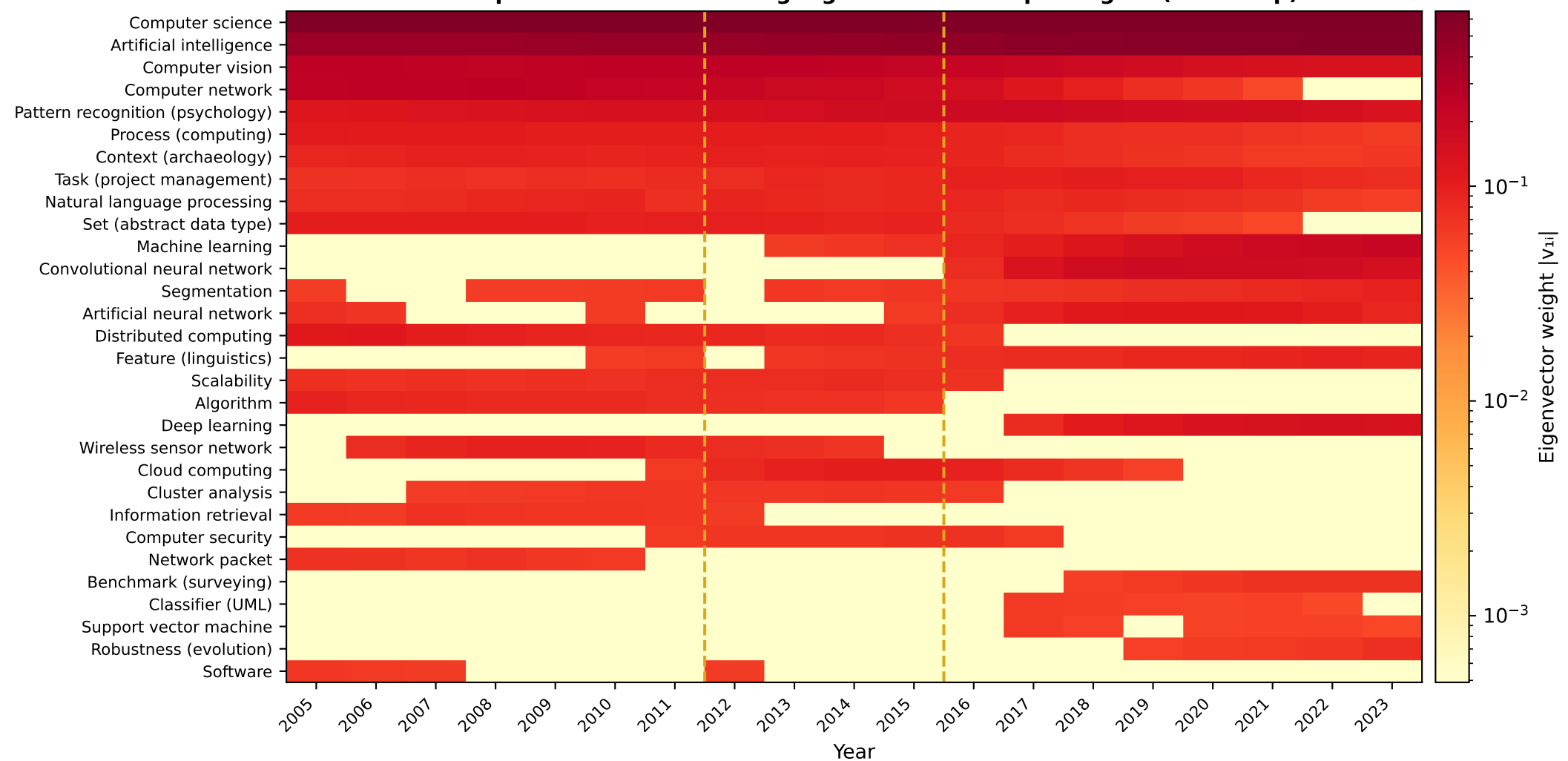
A Computer Science — leading eigenvector concept weights (heat-map)
