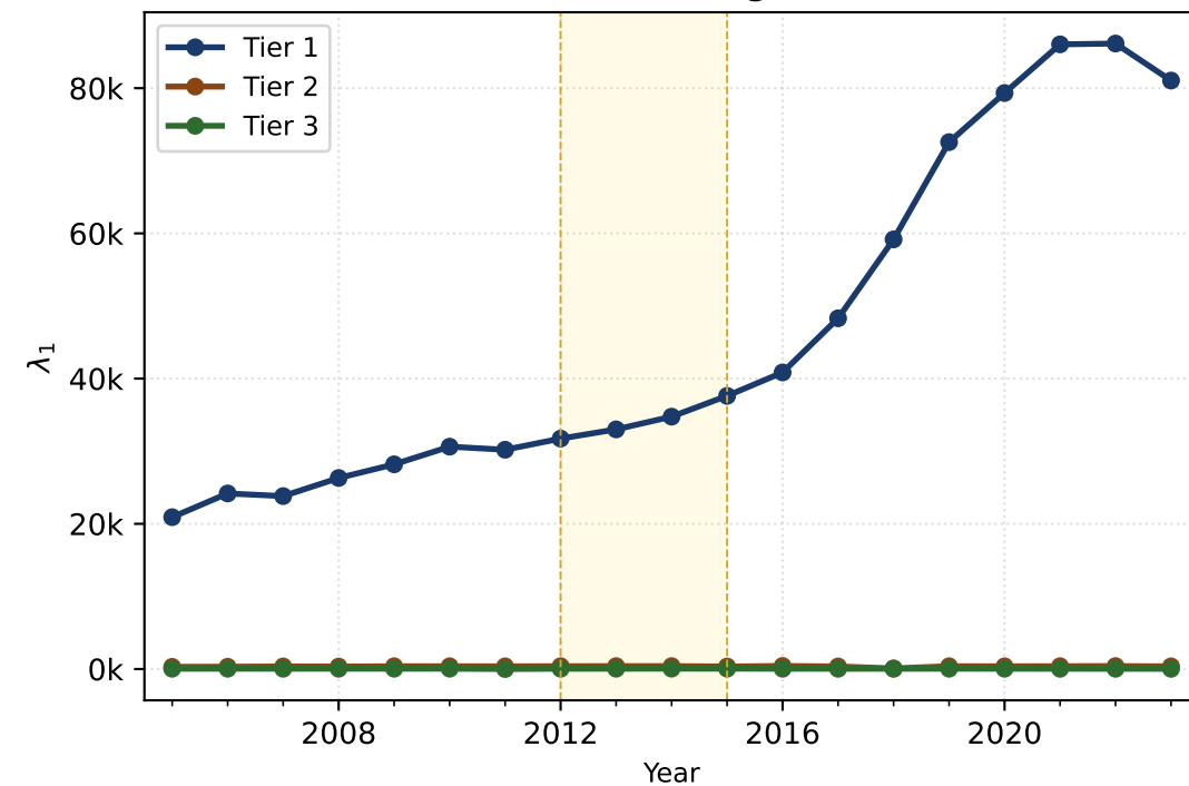
B Tier-resolved eigenvalues
