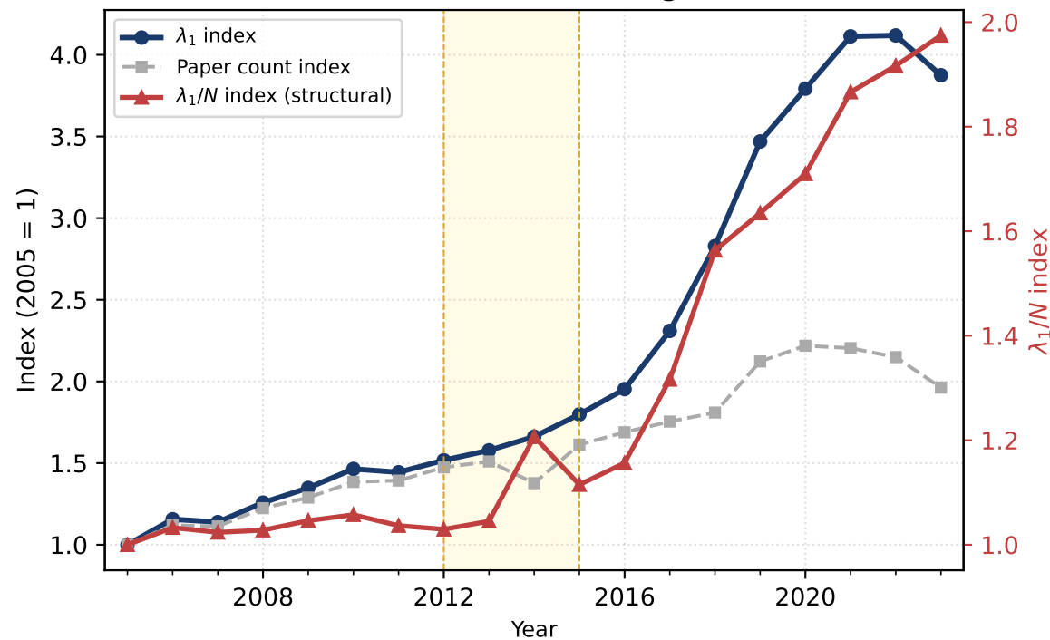
A Volume vs structural growth
