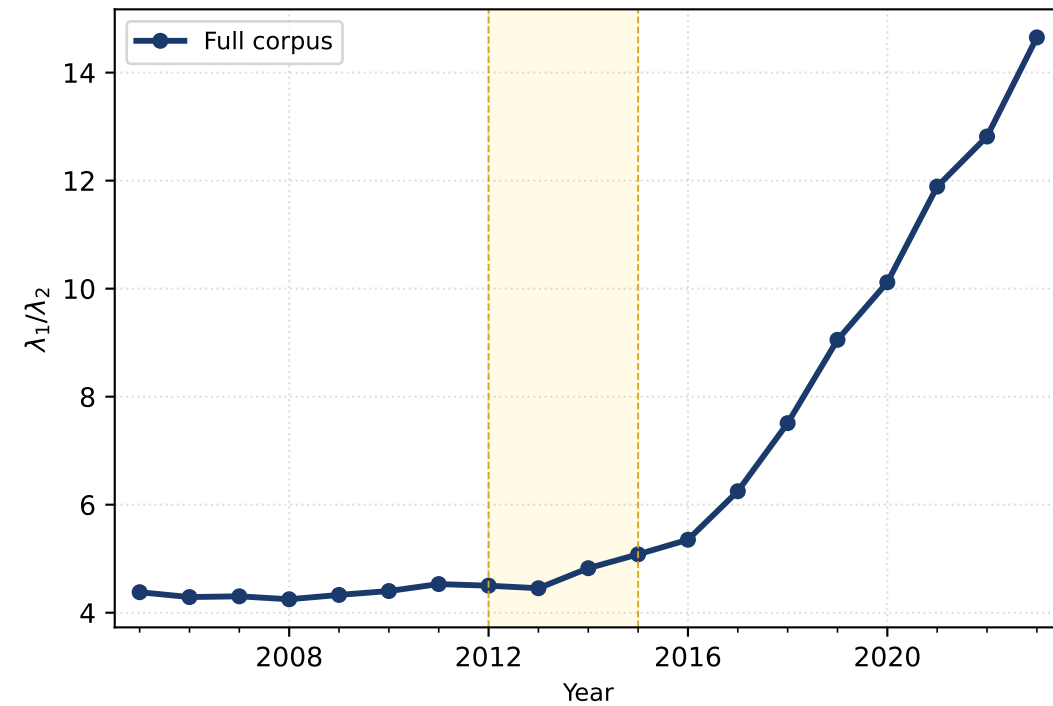
D Spectral gap (full corpus)
