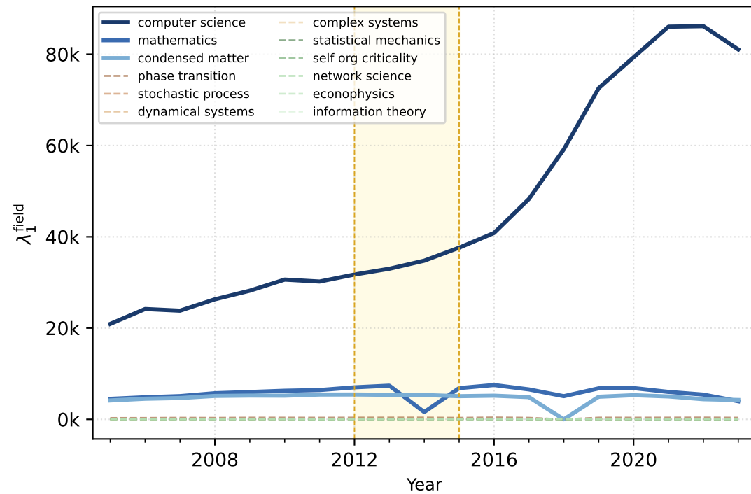
C Field-resolved eigenvalues
