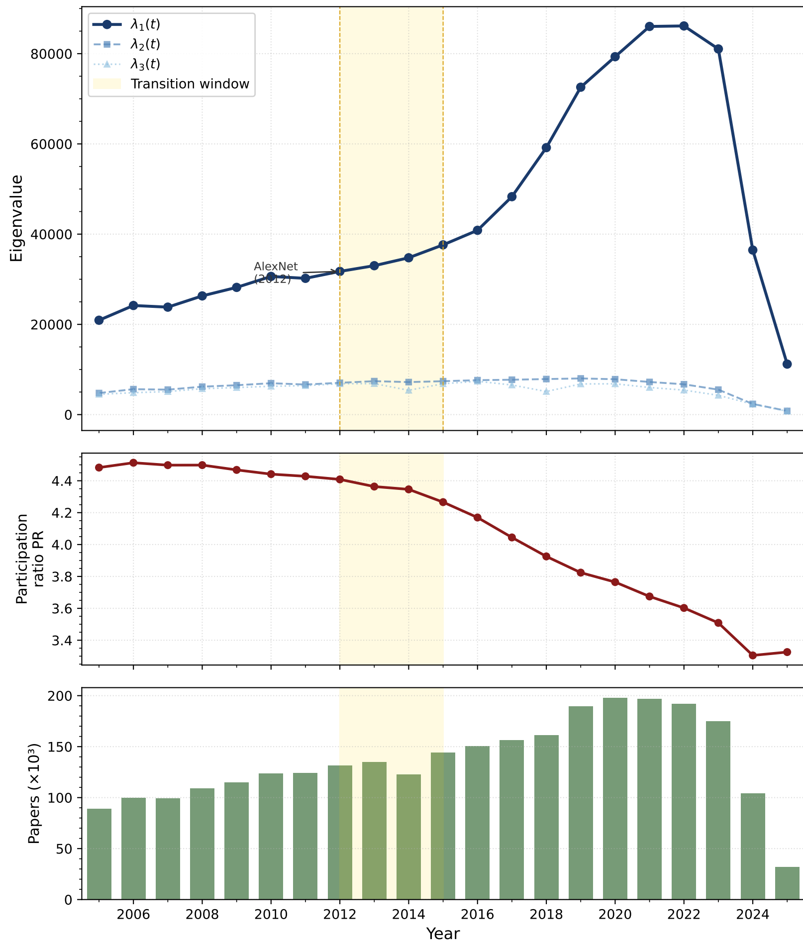
Leading eigenvalue \lambda_1(t) of concept co-occurrence matrix (deep learning paradigm transition)
