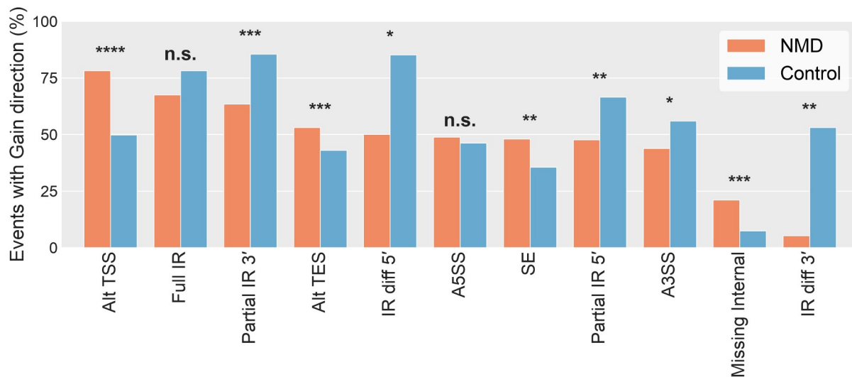
SF30 | Gain Direction by Splice Event Type. Percentage of detected splice events (across 1,548 gene-matched isoform triplets, both NMD and Control comparators) in which the comparator has additional sequence relative to its reference isoform (Gain direction). One bar-pair per event type — NMD comparators (orange) vs Control comparators (blue) — sorted by NMD-side %Gain, descending. Direction is defined from the comparator's perspective (see SF25 for event-type definitions). Significance stars, Fisher's exact test on the 2 \times 2 (Gain/Loss \times NMD/Control) count table per event type: * p < 0.05 , ** p < 10^{-3} , *** p < 10^{-4} , **** p < 10^{-10} ; n.s. otherwise.
