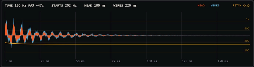
808 Snare. Two tones and a little noise.
