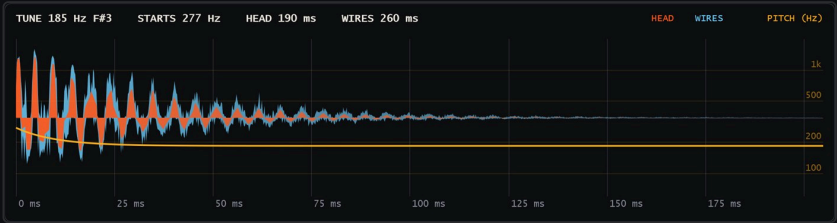
909 Snare. Triangles, the drop, bright noise.
