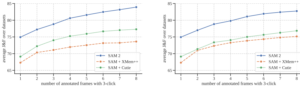
Figure 5 Zero-shot accuracy over 9 datasets in interactive offline and online evaluation settings.
