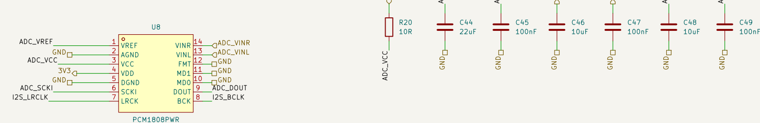
F. Audio in: PCM1808 on SAI1 block B, slave on BCLK/LRCLK. VINL/VINR arrive AC-coupled from the top sheet
