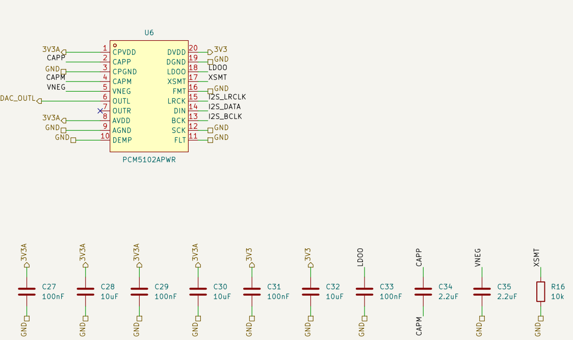
D. Audio out: PCM5102A, OUTL leaves on DAC_OUTL, OUTR unused
