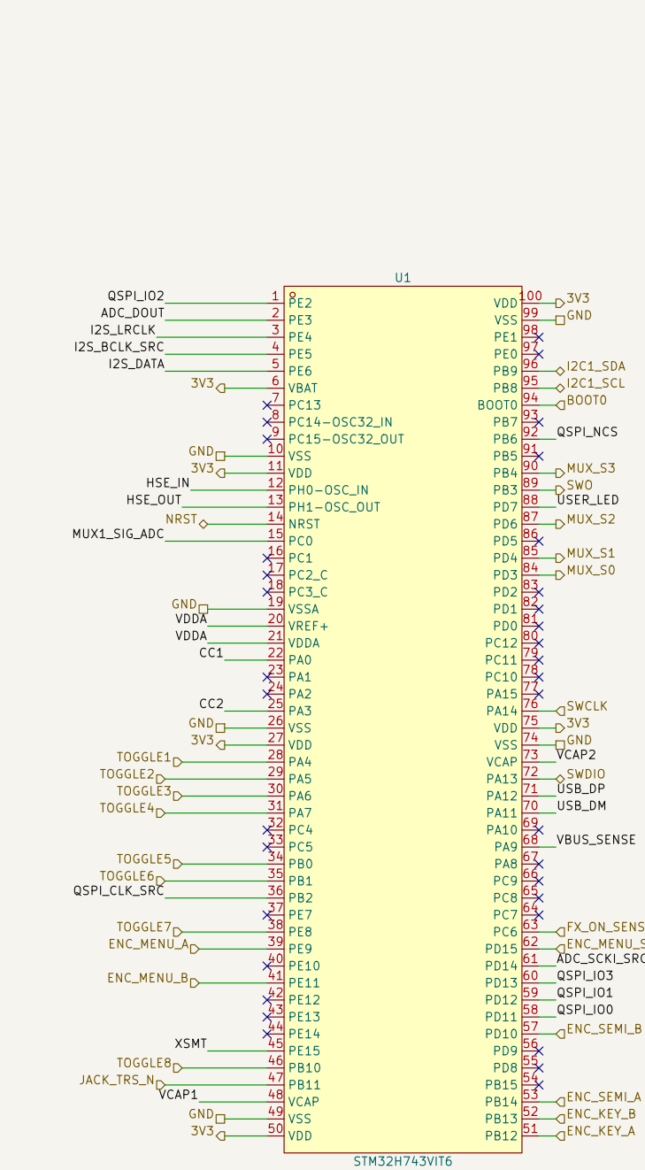
A. Compute core: U1 and its decoupling, HSE, reset, BOOT0, user LED
