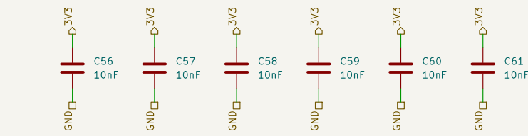
G. Reference-transition stitching, 10 nF 3V3-GND, one per via group:
