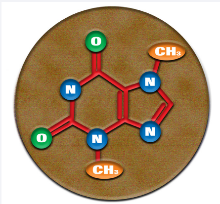
THEOBROMINE
