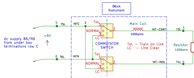
Block Shelf – Rear Terminal Strip
