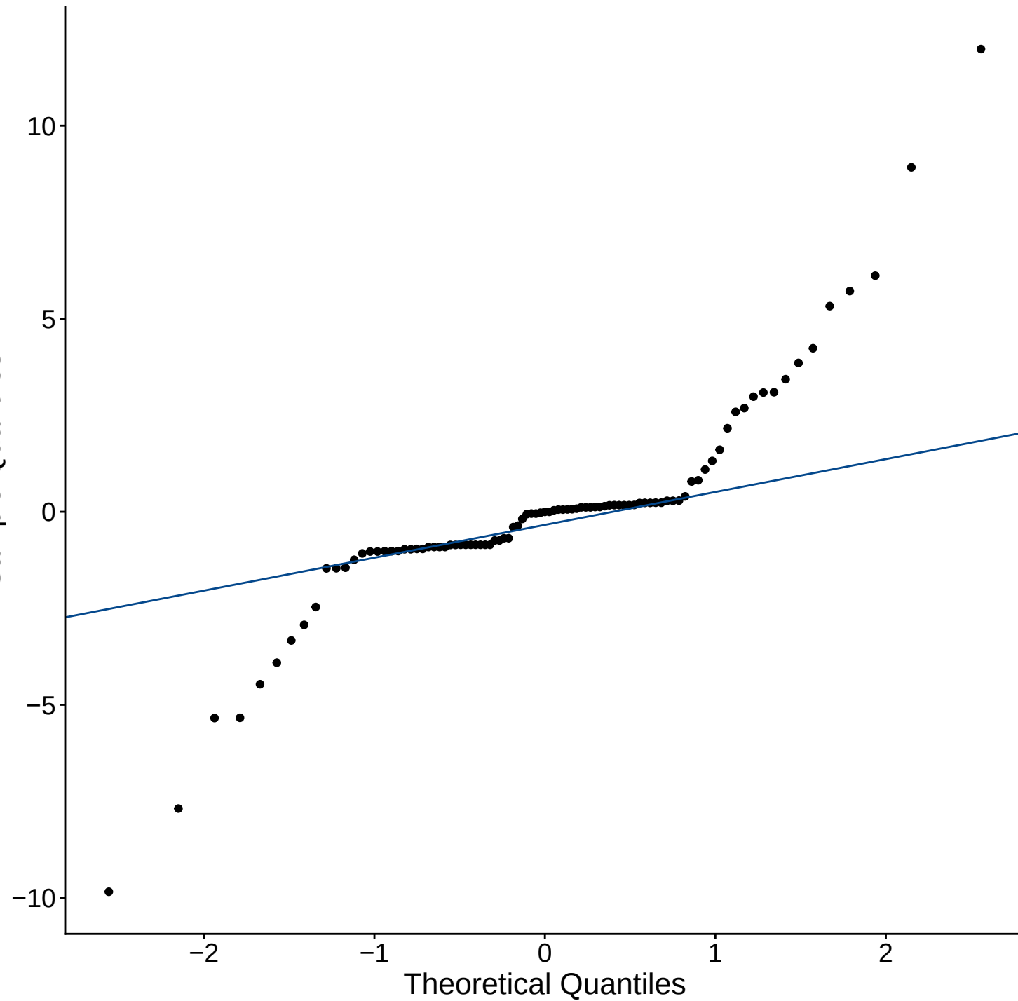
Q-Q Plot
