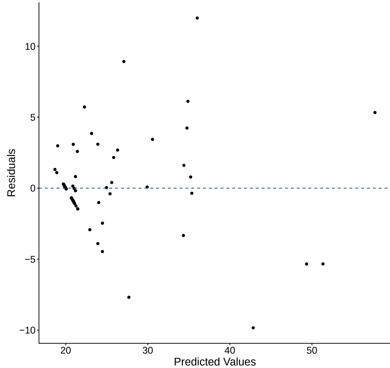
Residual Plot
