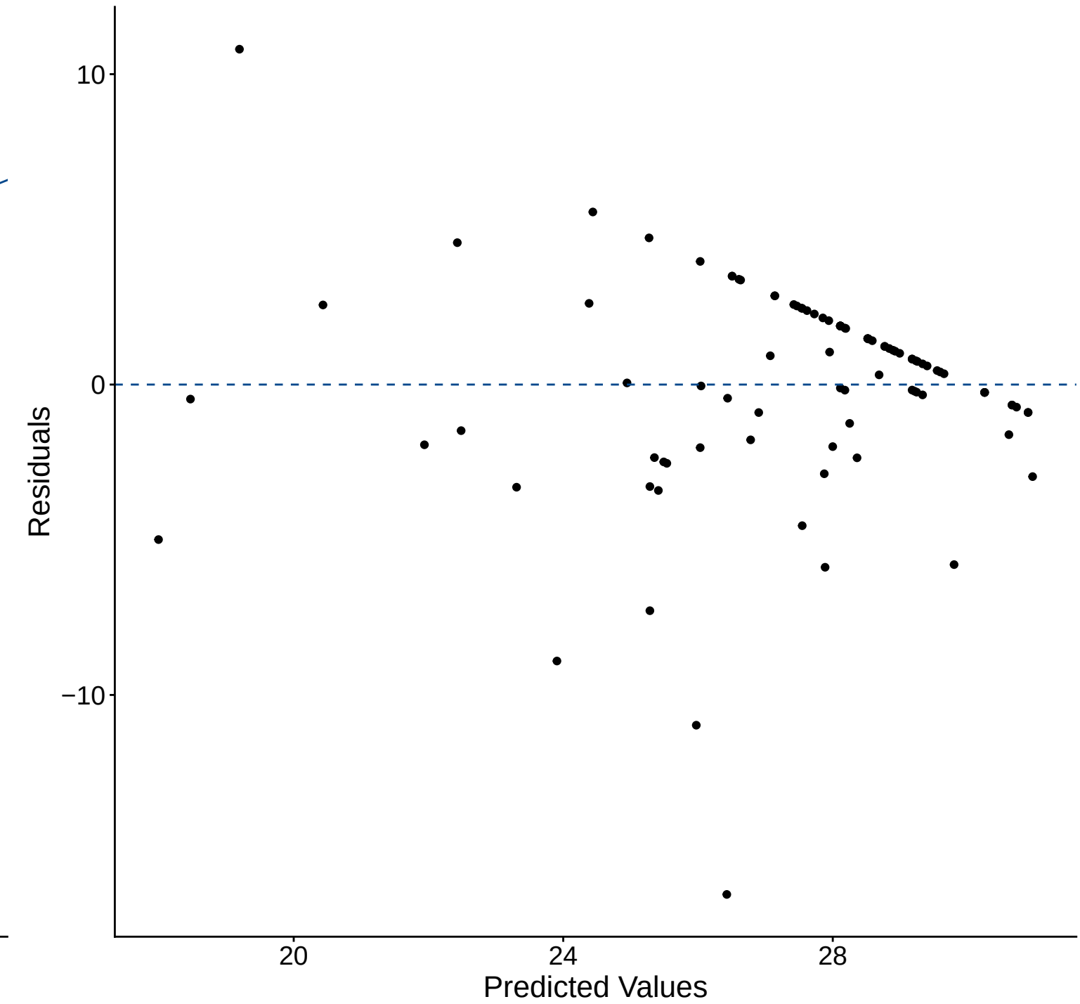
Residual Plot
