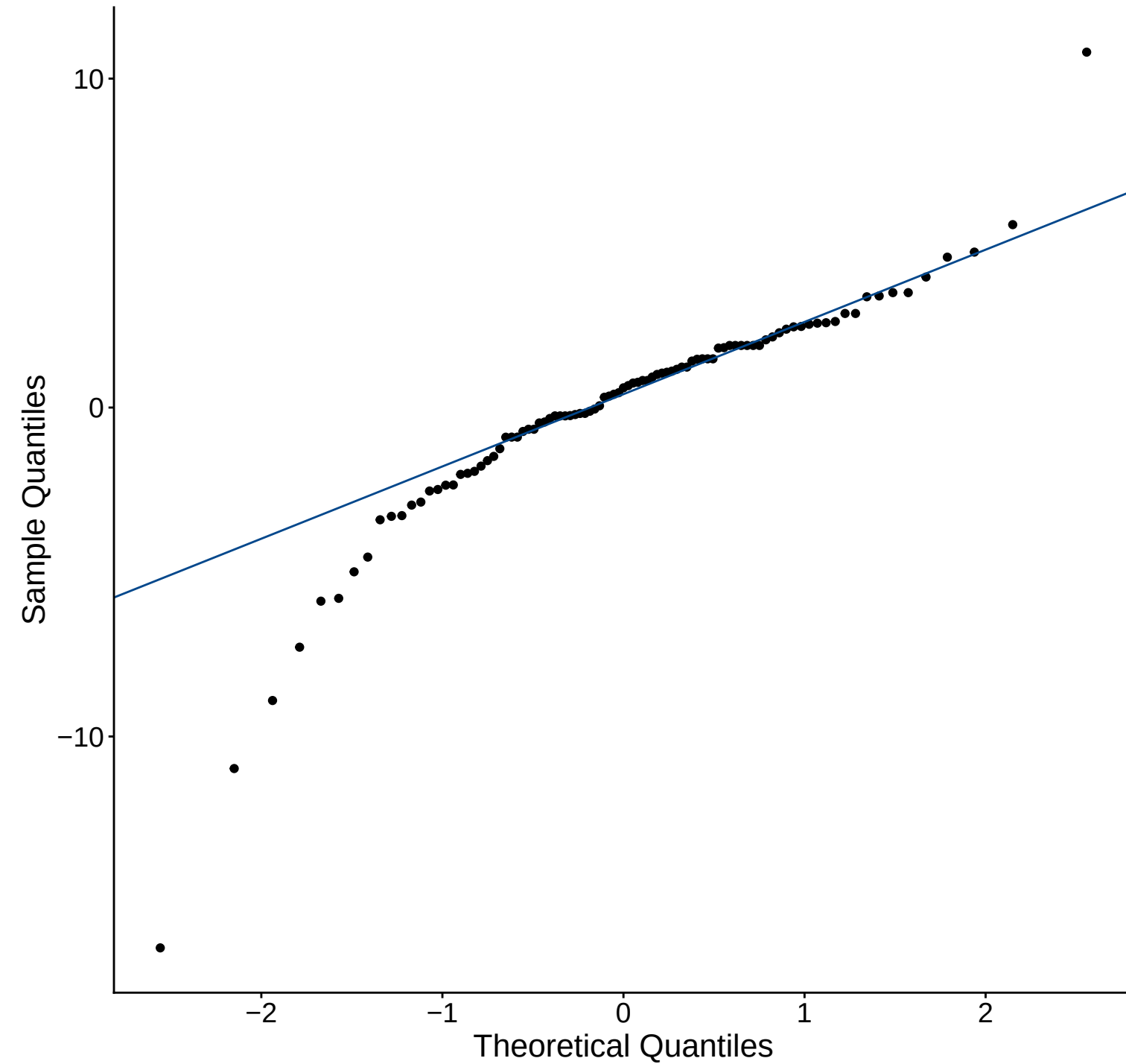
Q-Q Plot
